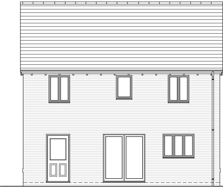
Rear Elevation
