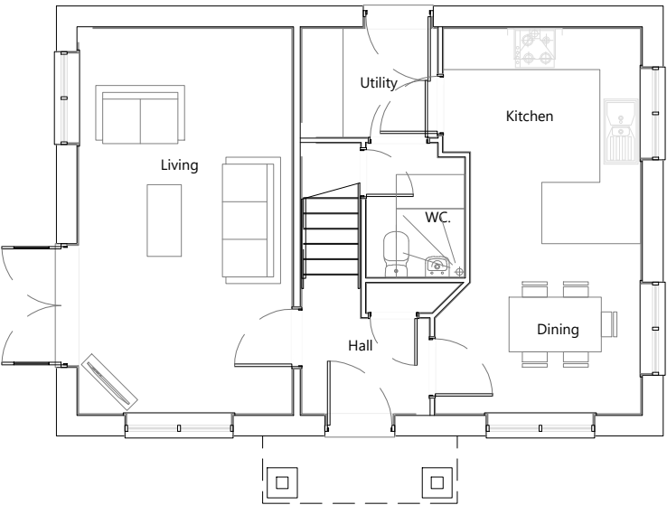
Ground Floor Plan Plot 242 - Barnwood SR2
