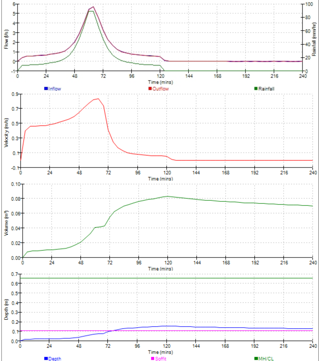
Graphs for Pipe 1.002 US/MH S3 (Storm) 120 minute 100 year Summer Status: SURCHARGED
