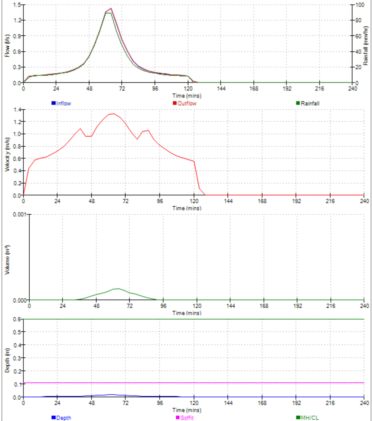
Graphs for Pipe 2.000 US/MH RE2 (Storm) 120 minute 100 year Summer Status: OK
