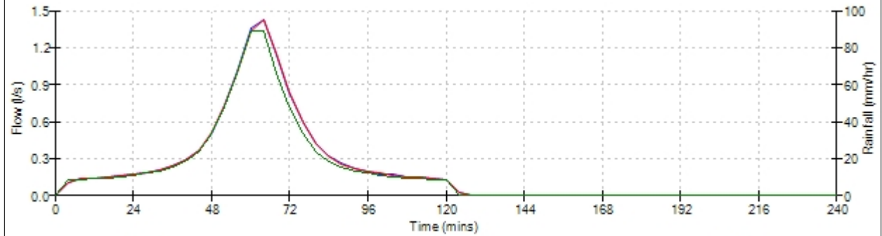
Graphs for Pipe 1.000 US/MH RE1 (Storm) 120 minute 100 year Summer Status: OK
