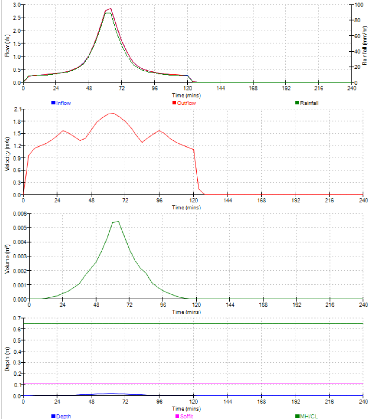
Graphs for Pipe 2.001 US/MH S2 (Storm) 120 minute 100 year Summer Status: OK
