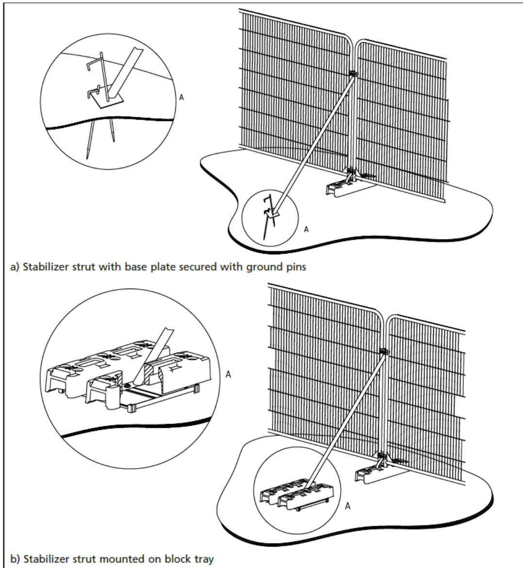
Figure 2 Tree Protection Fencing Design for Hard Surfaces Only (BS5837 2012)
