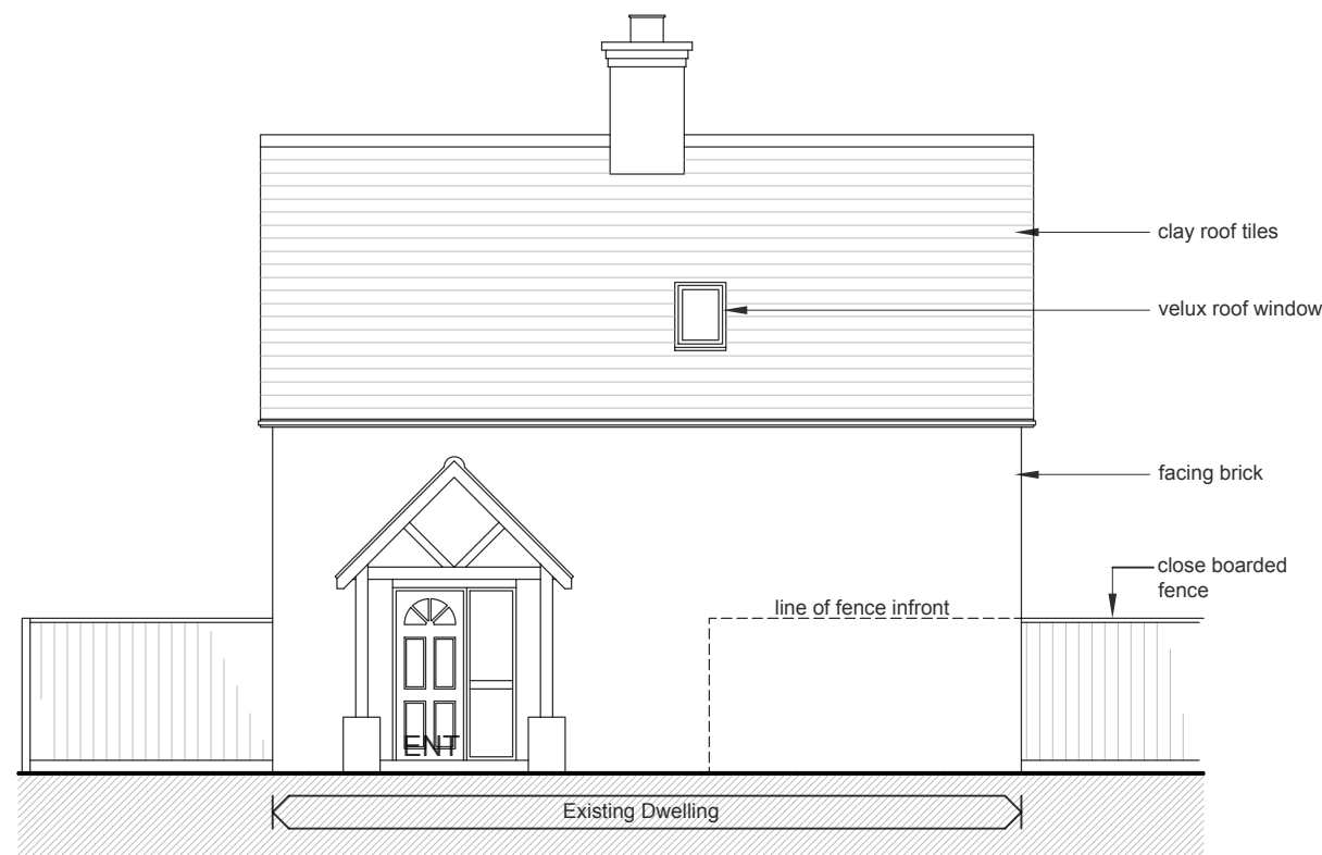
95c EAST ELEVATION
