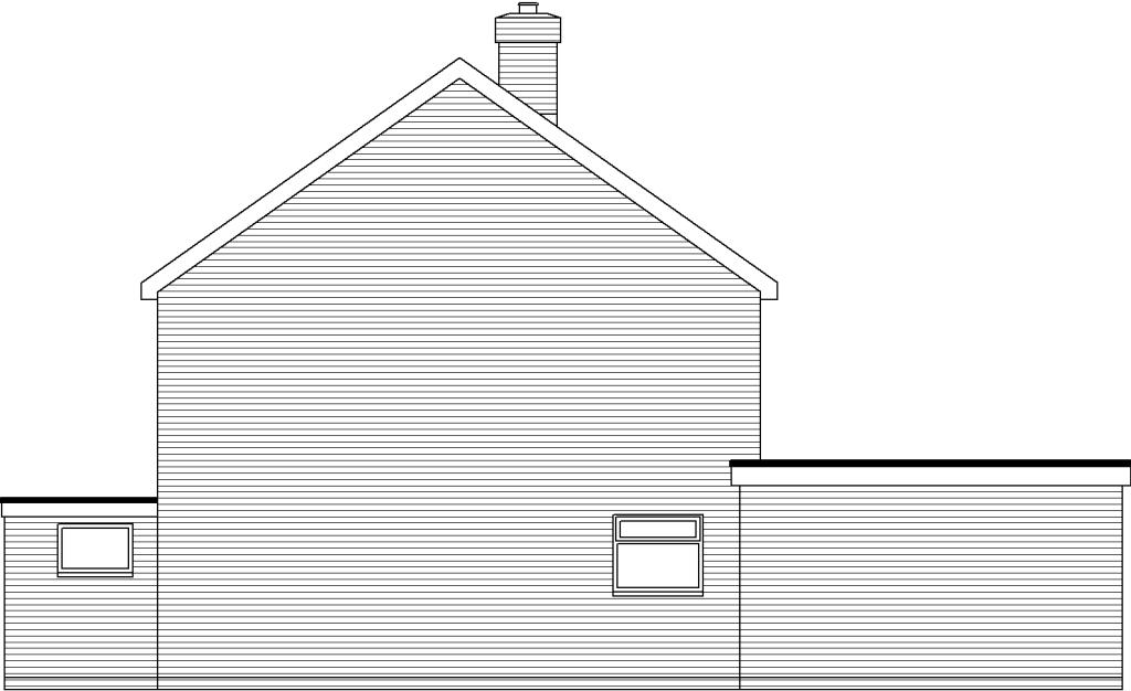
EXISTING SIDE ELEVATION SCALE 1/50 ON A3
