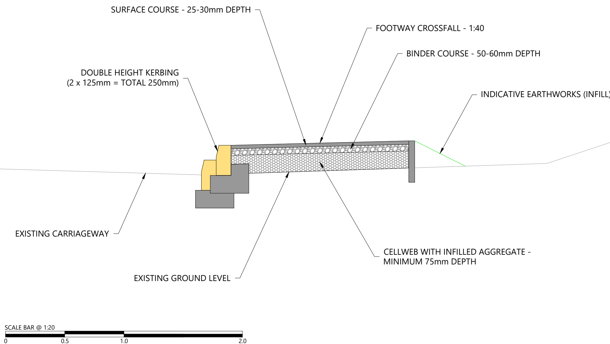
INDICATIVE NO-DIG FOOTWAY CONSTRUCTION DETAIL
