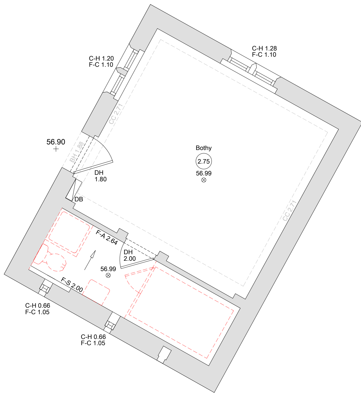
GROUND FLOOR GENERAL ARRANGEMENT - DETACHED BOTHY AS PROPOSED SCALE @ 1:50 ON AN A1 SHEET
