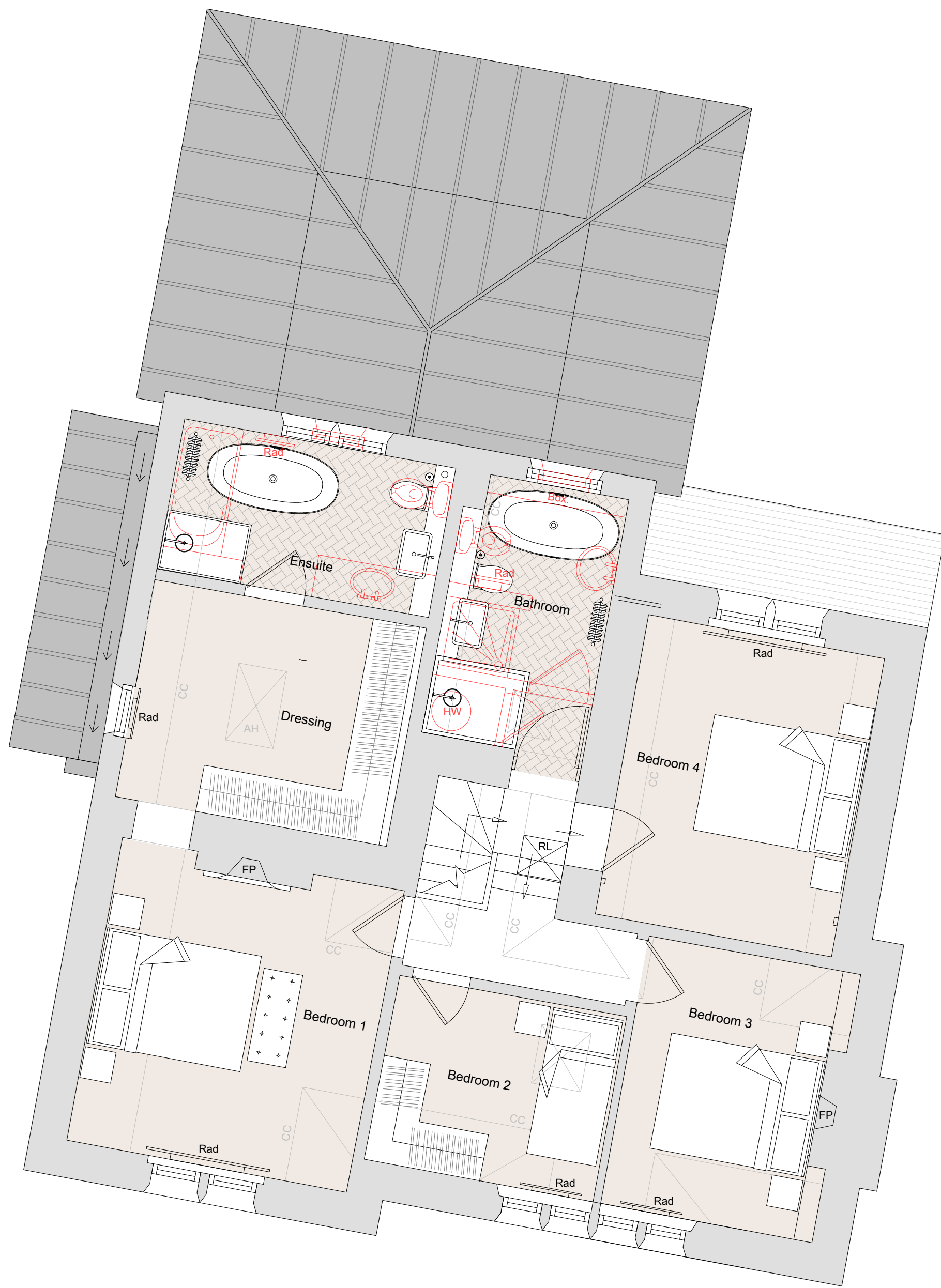
FIRST FLOOR GENERAL ARRANGEMENT - AS PROPOSED SCALE @ 1:50 ON AN A1 SHEET
