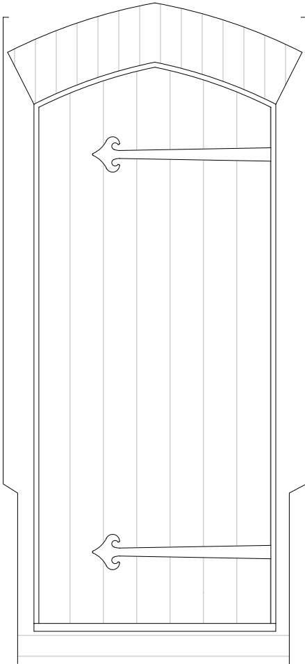
Door - Outside face 1:20 PROPOSED
