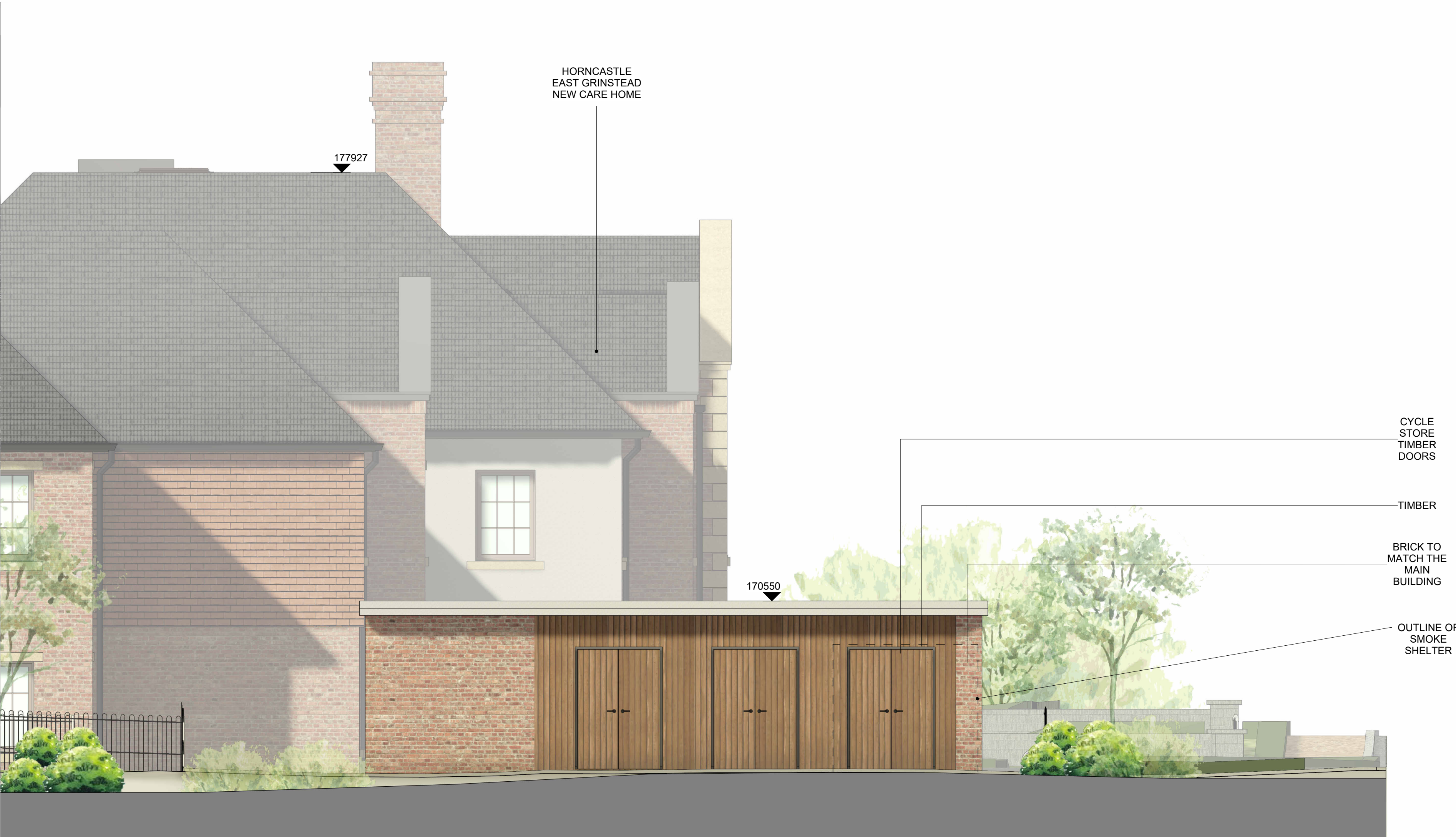
B. EAST ELEVATION 1 : 50
