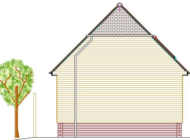
Northern Elevation
