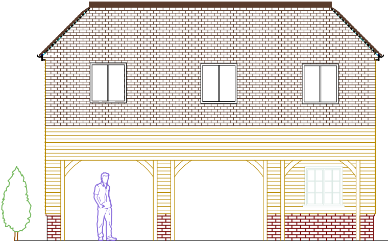
Western Elevation
