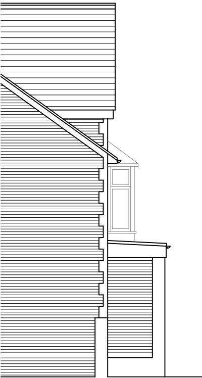
East Elevation as Existing
