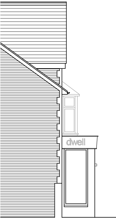
East Elevation as Proposed
