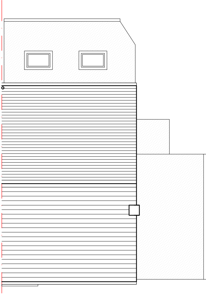
ROOF PLAN
