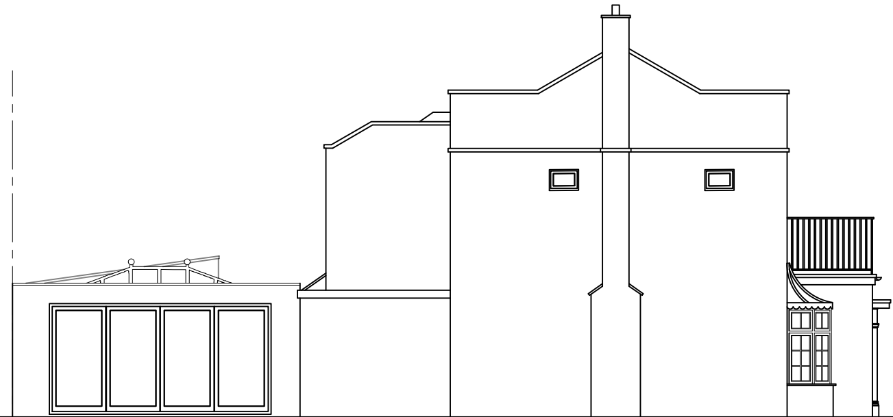
Side Elevation 1:100
