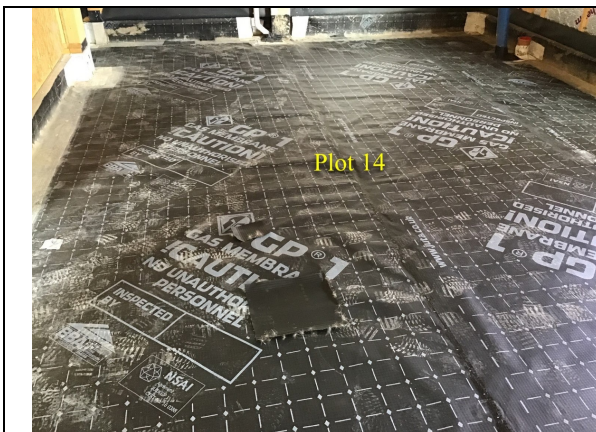
Overview of the Juta GP1 Gas Membrane that has been installed as an infill to plot 14.
