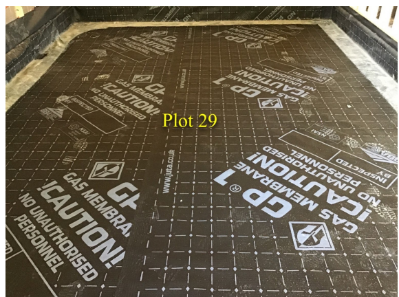
Overview of the Juta GP1 Gas Membrane that has been installed as an infill to plot 29.
