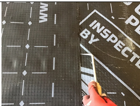
Plot 23 hand welded membrane lap testing.
