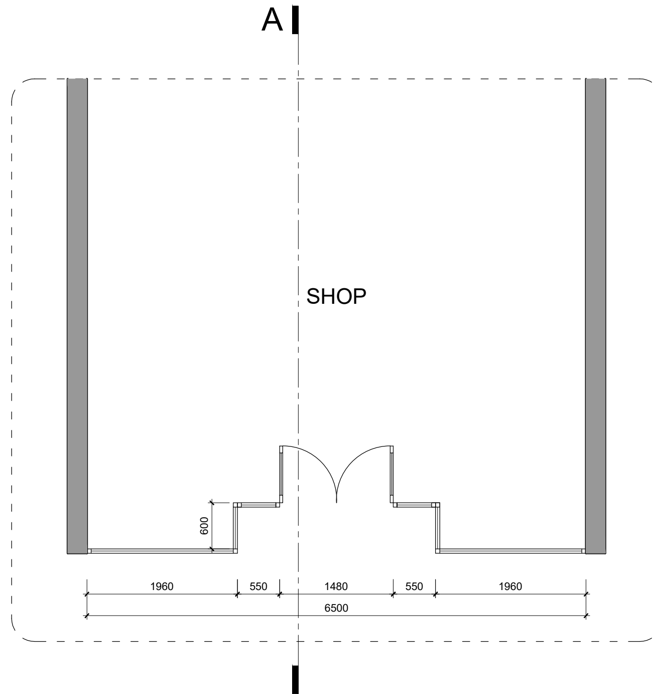
PROPOSED LAYOUT
