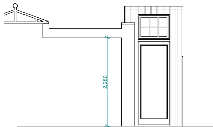
FRONT ELEVATION OF UTILITY DOOR SCALE 1.100
