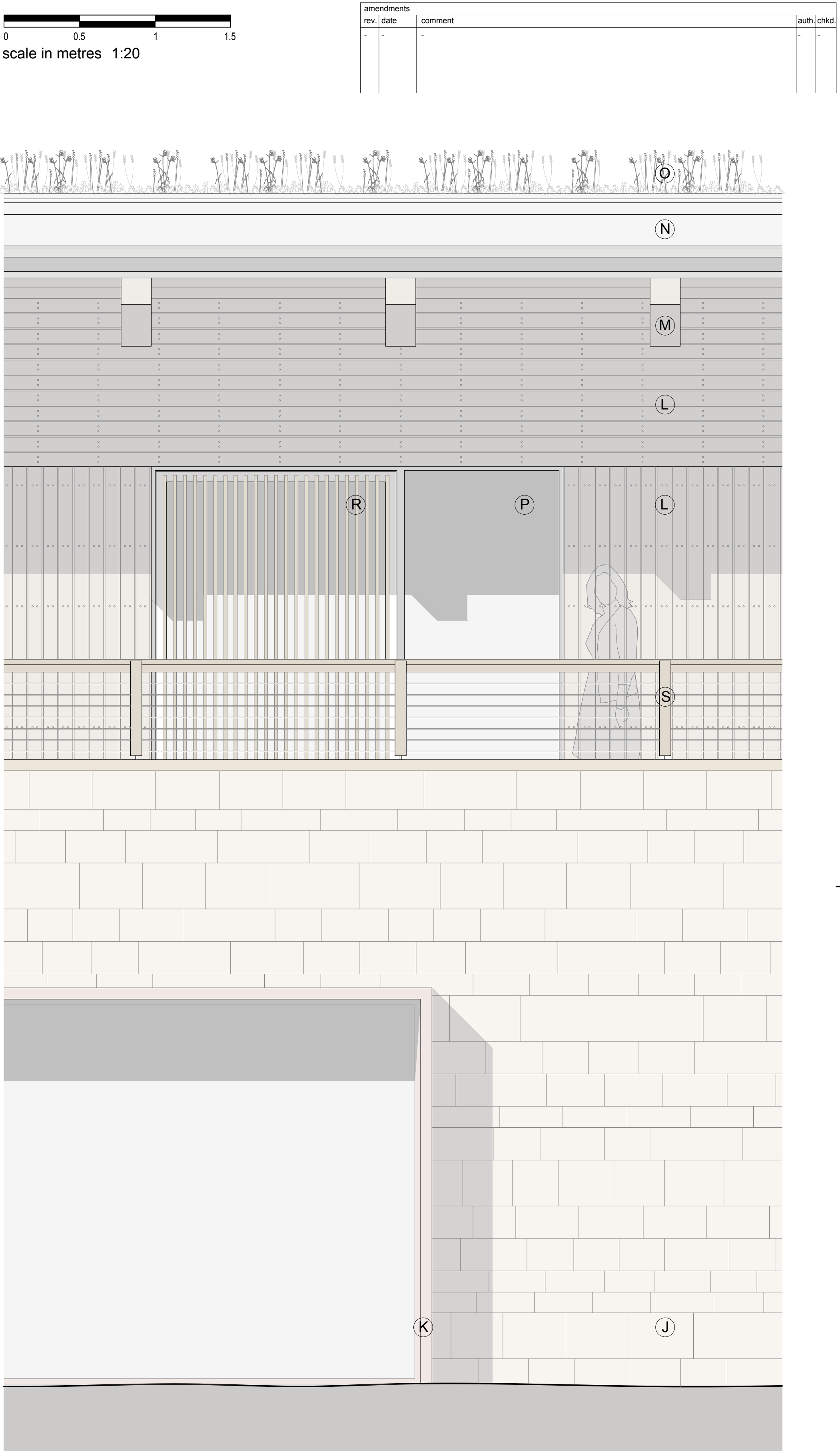
Proposed Detail Elevation 1:20
