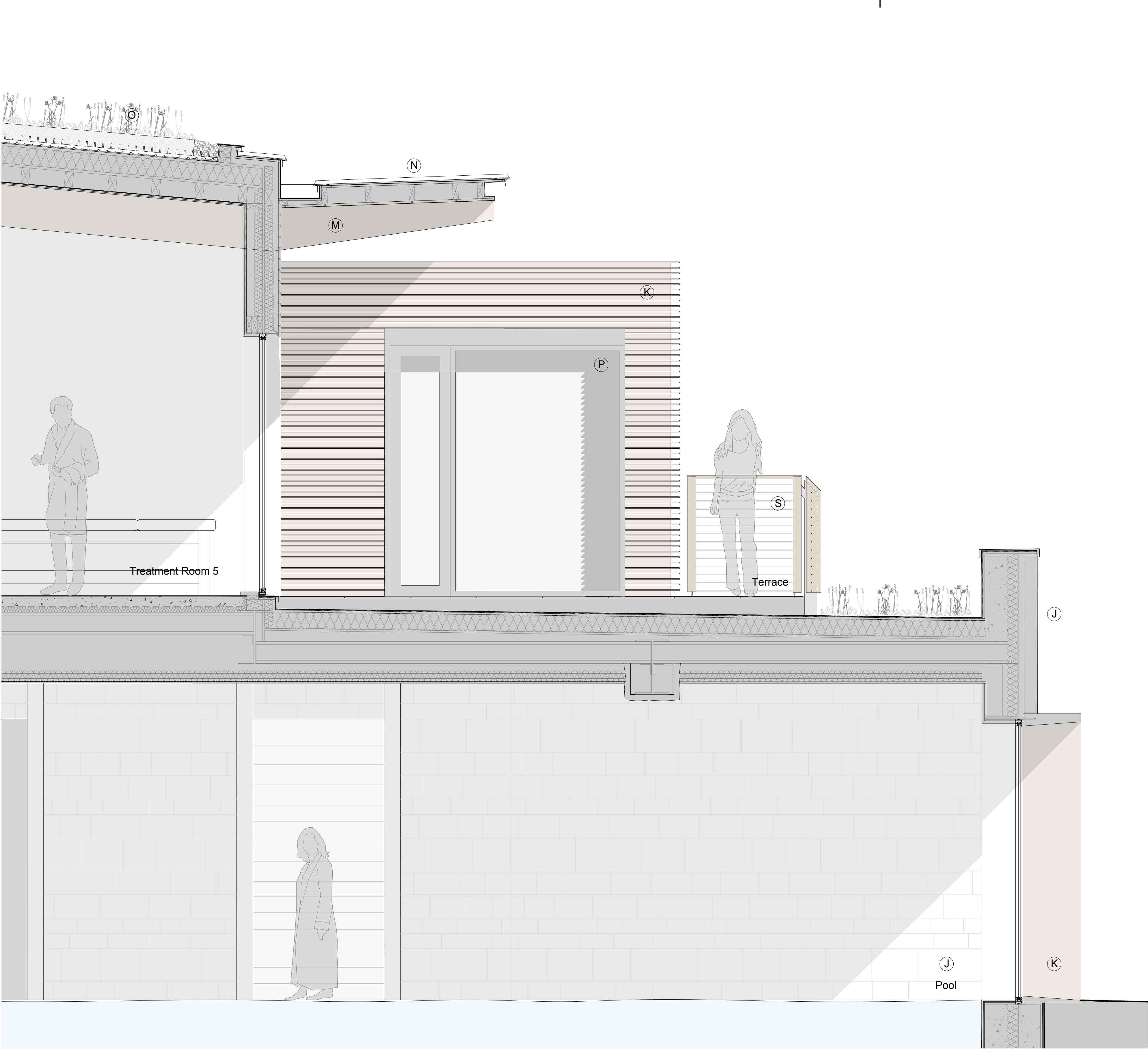
Proposed Detail Section 1:20
