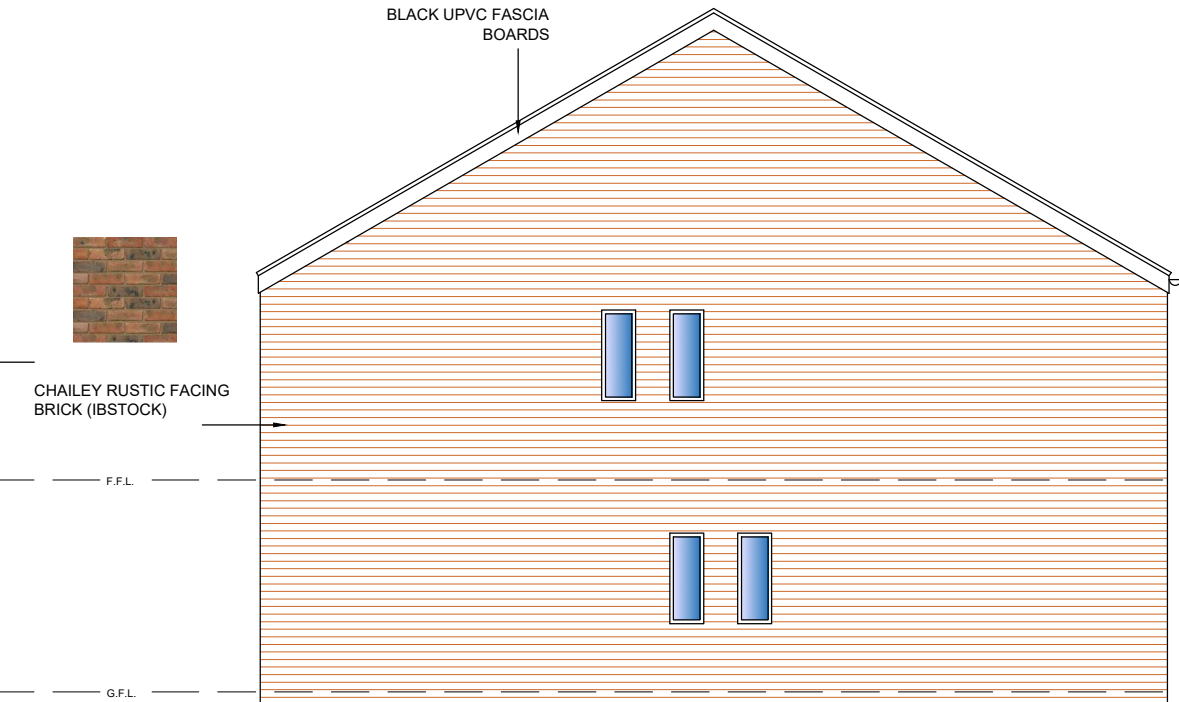
PLOT ONE PROPOSED REAR ELEVATION
