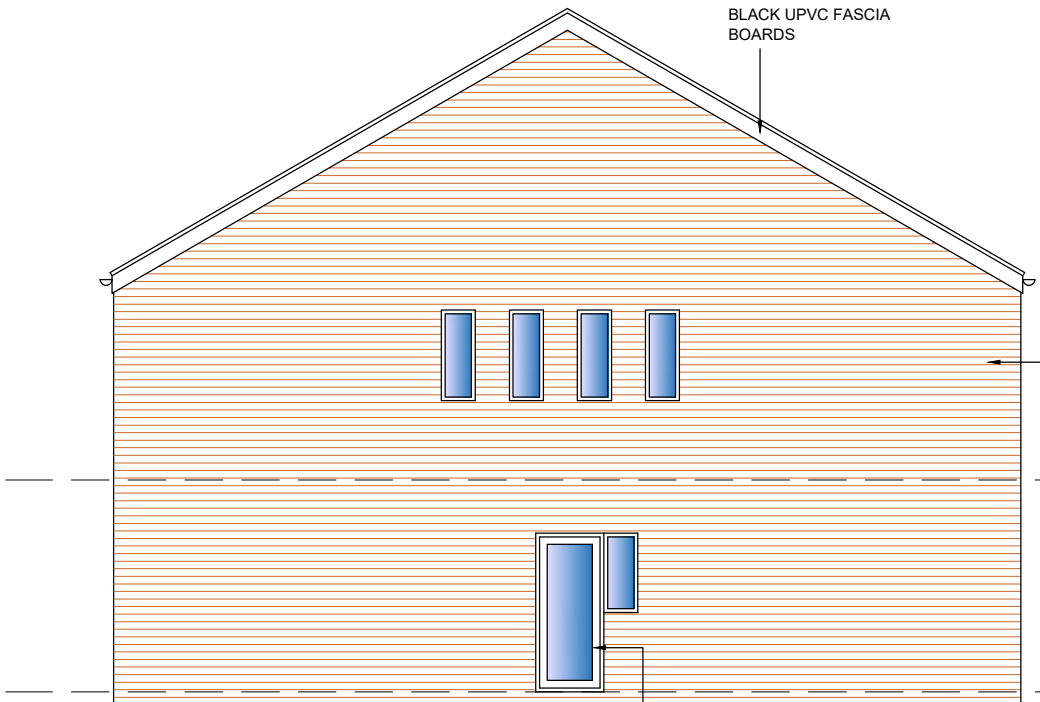
PLOT ONE PROPOSED FRONT ELEVATION
