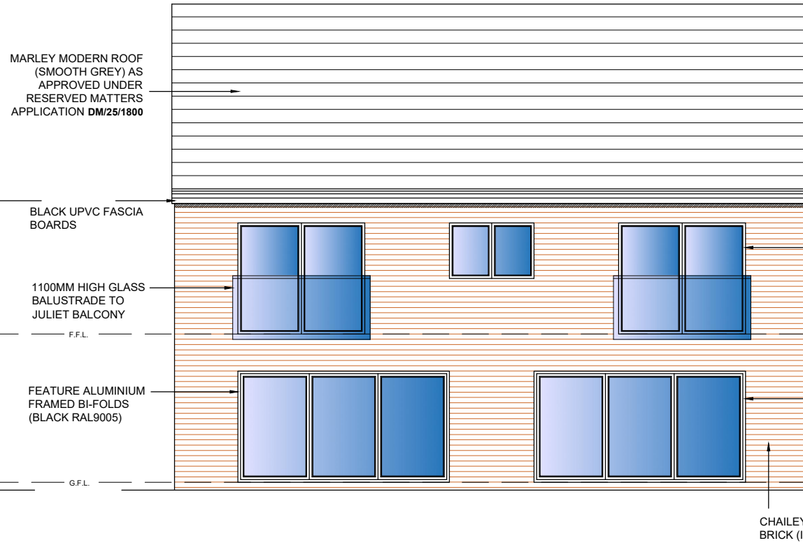
PLOT TWO PROPOSED REAR ELEVATION
