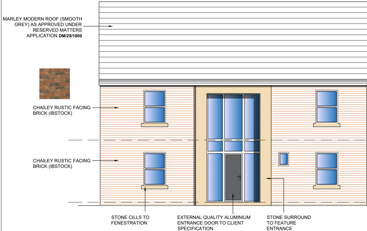
PLOT TWO PROPOSED FRONT ELEVATION
