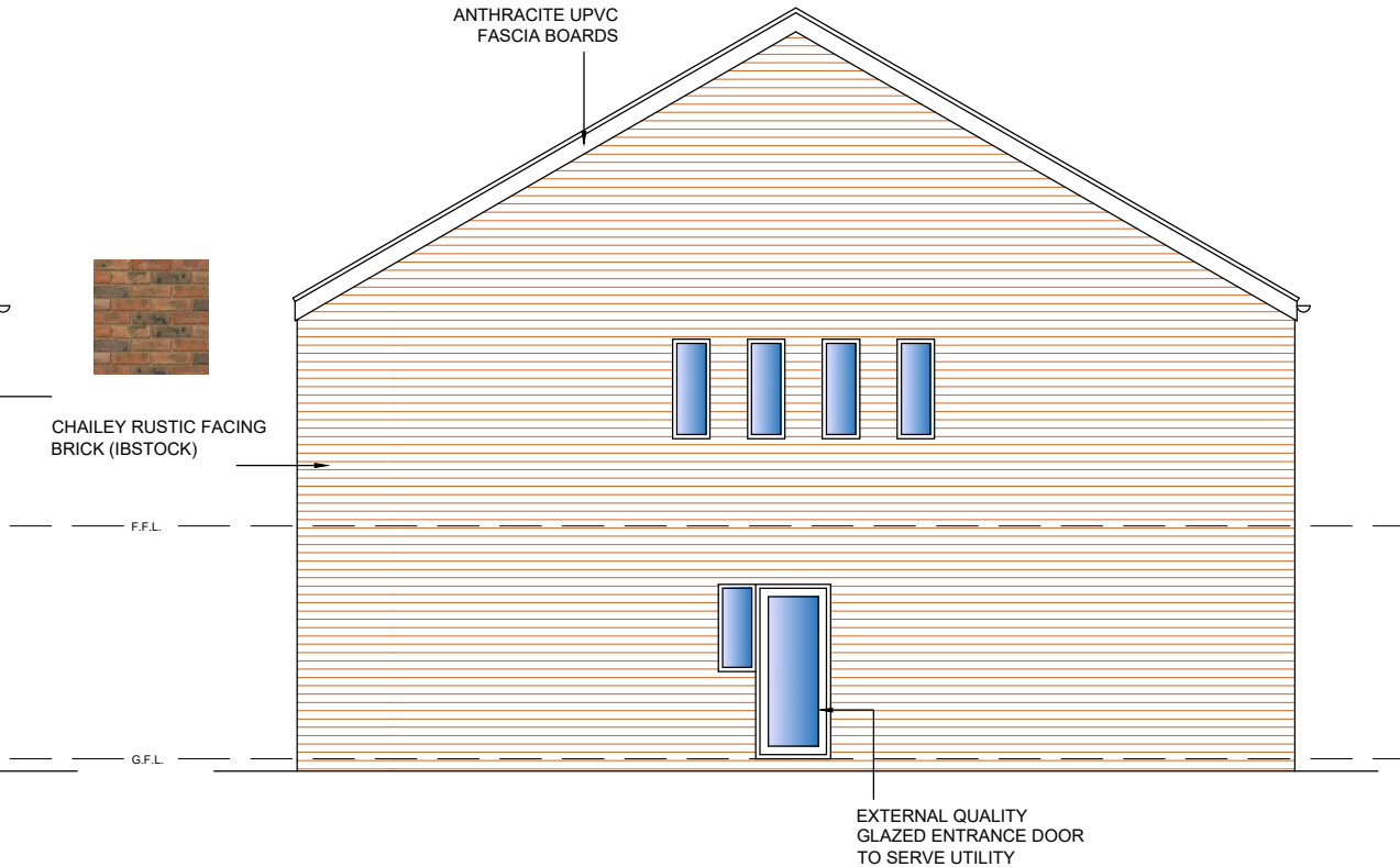
PLOT TWO PROPOSED SIDE ELEVATION
