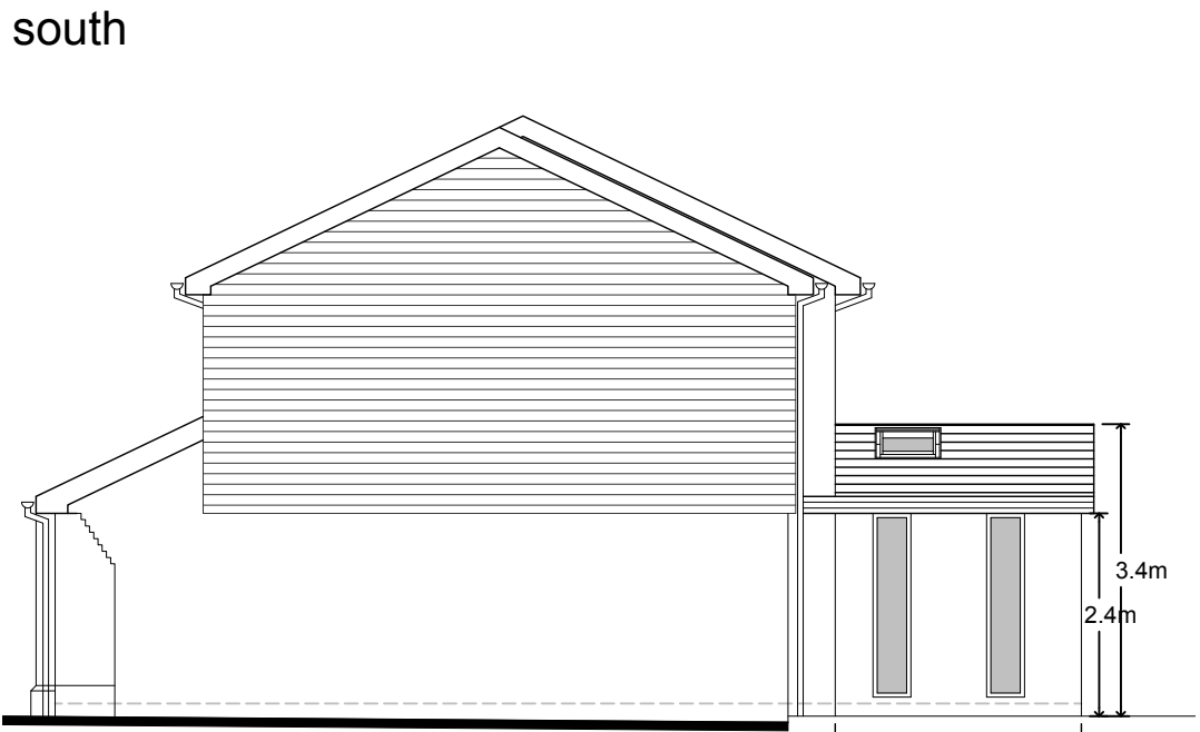
new single storey rear extension
