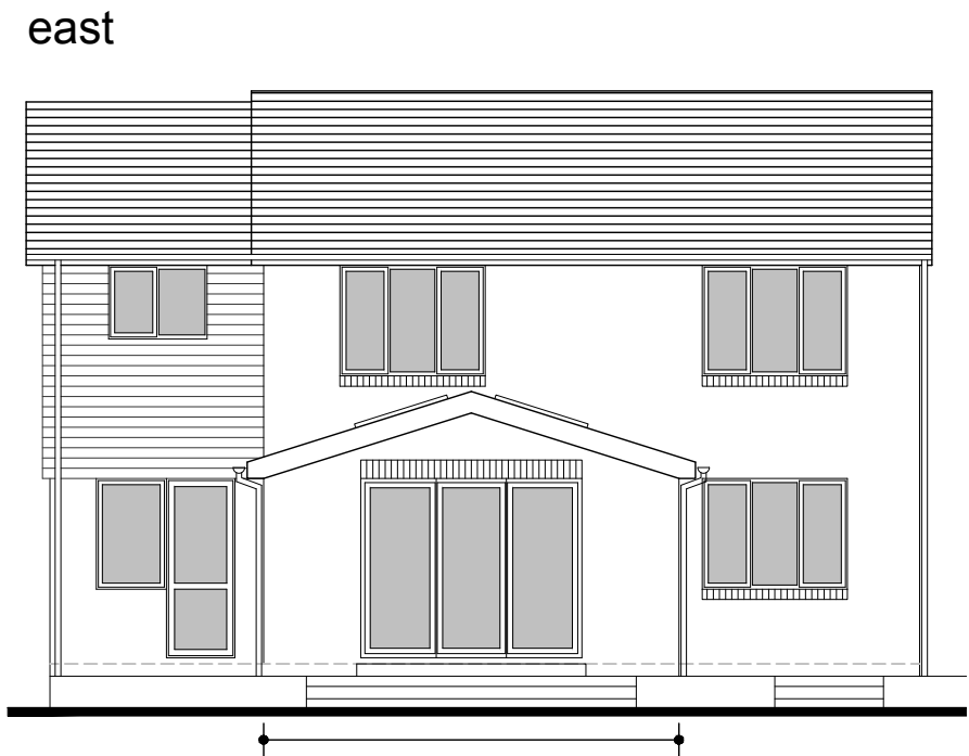
new single storey rear extension
