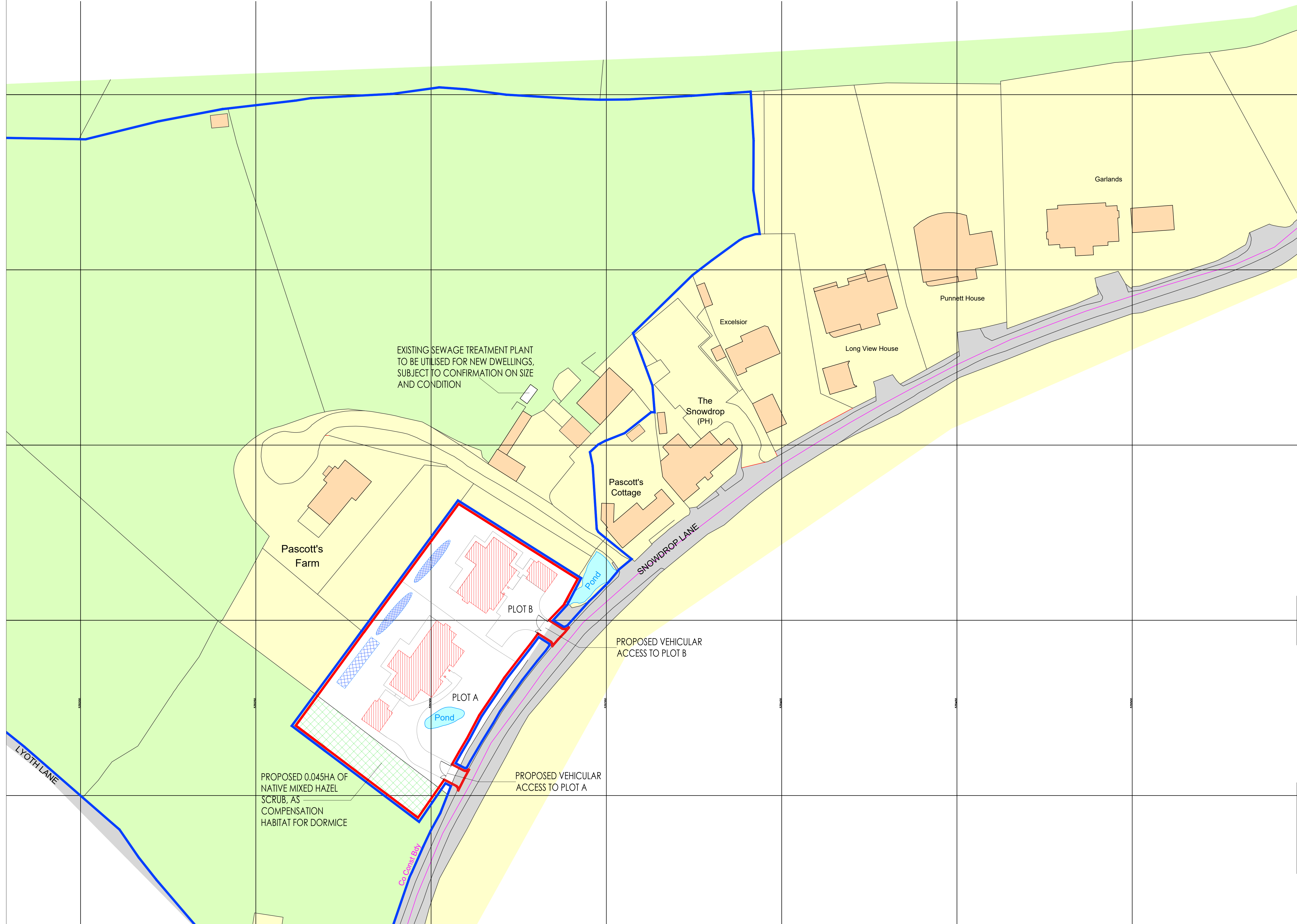
SITE BLOCK PLAN - AS PROPOSED SCALE @ 1:500 ON AN A1 SHEET
