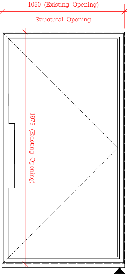
ED.001 Aluminium Crittal Style Door, set behind stable door.
