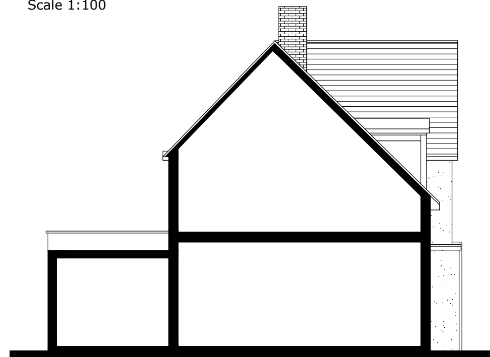
Existing Side Section / Elevation Scale 1:100
