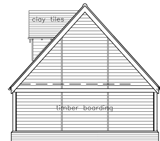
south elevation
