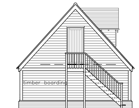
north elevation
