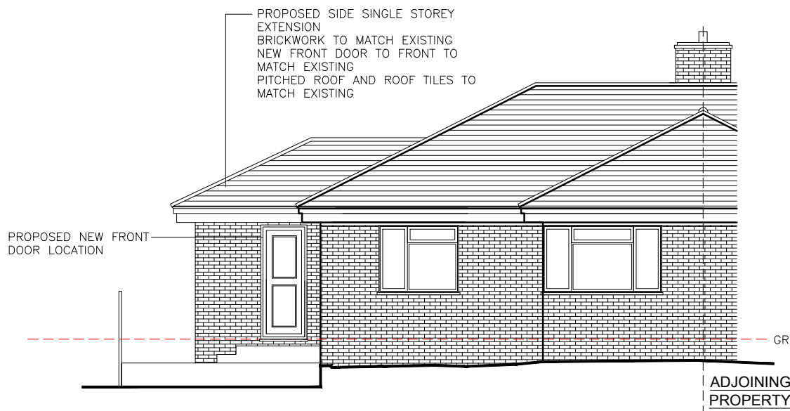
A) Proposed Front Elevation
