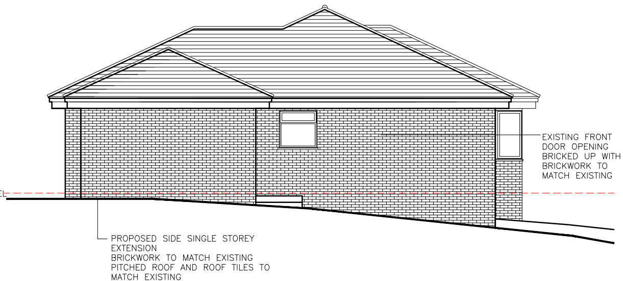
B) Proposed Side Elevation
