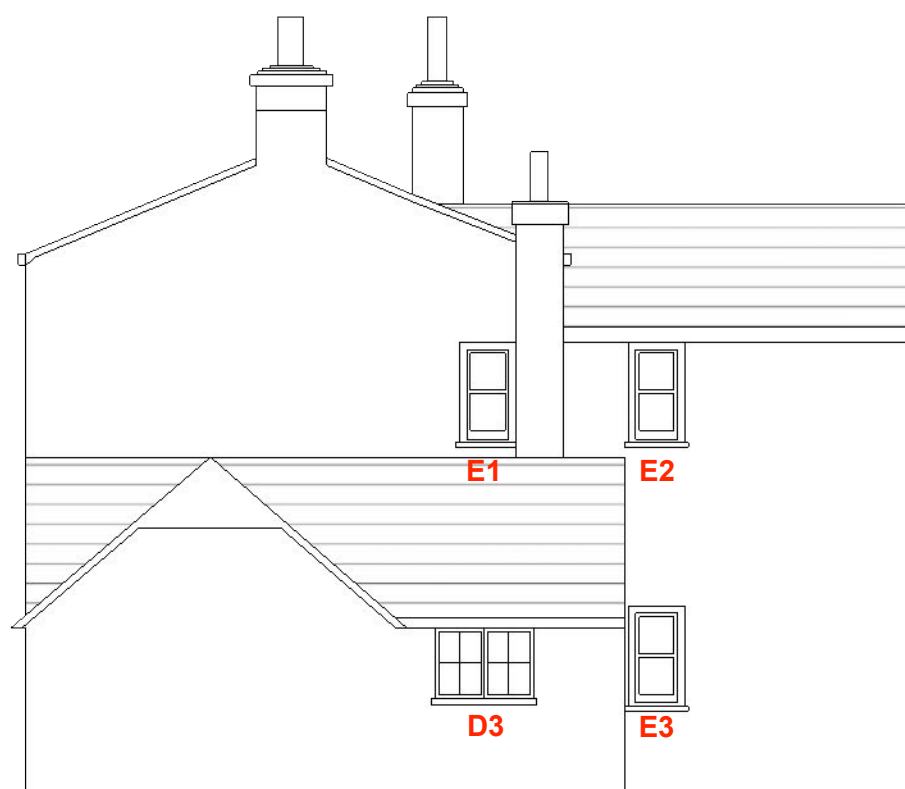
SIDE ELEVATION (NORTH)
