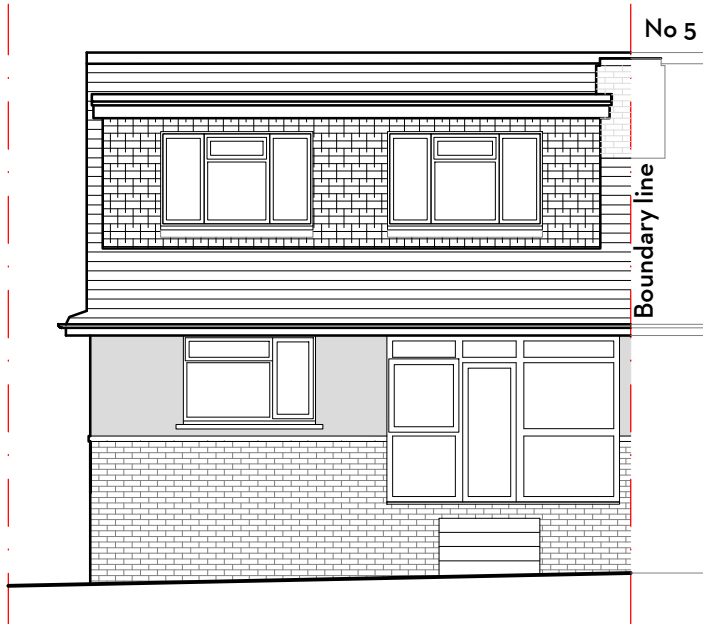
SOUTH ELEVATION
