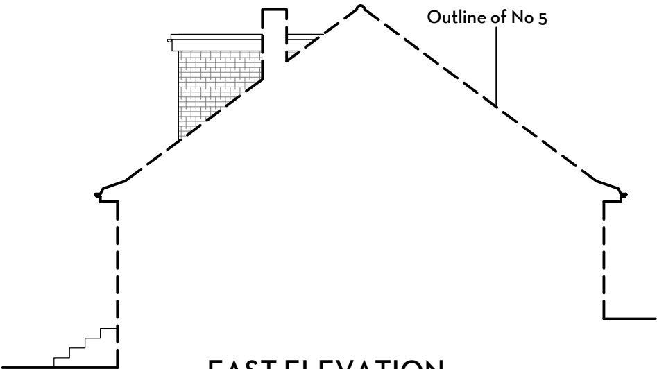
EAST ELEVATION
