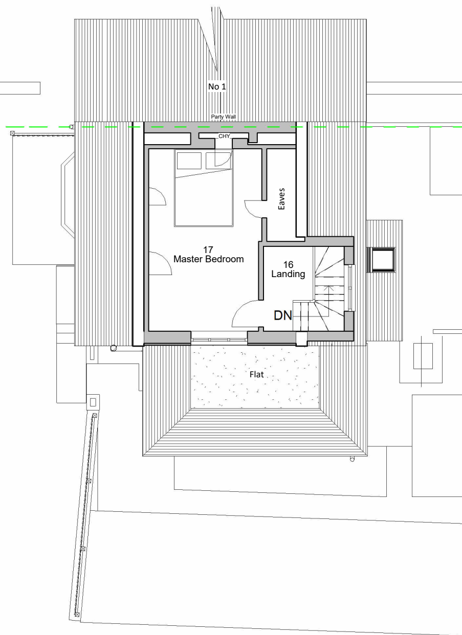
3 Existing Second floor 1 : 100
