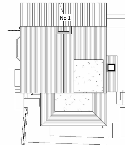
4 Existing Roof 1 : 200
