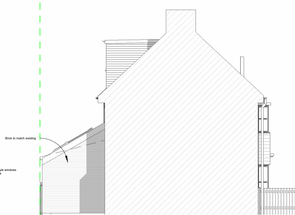
3 Proposed South Elevation 1 : 100
