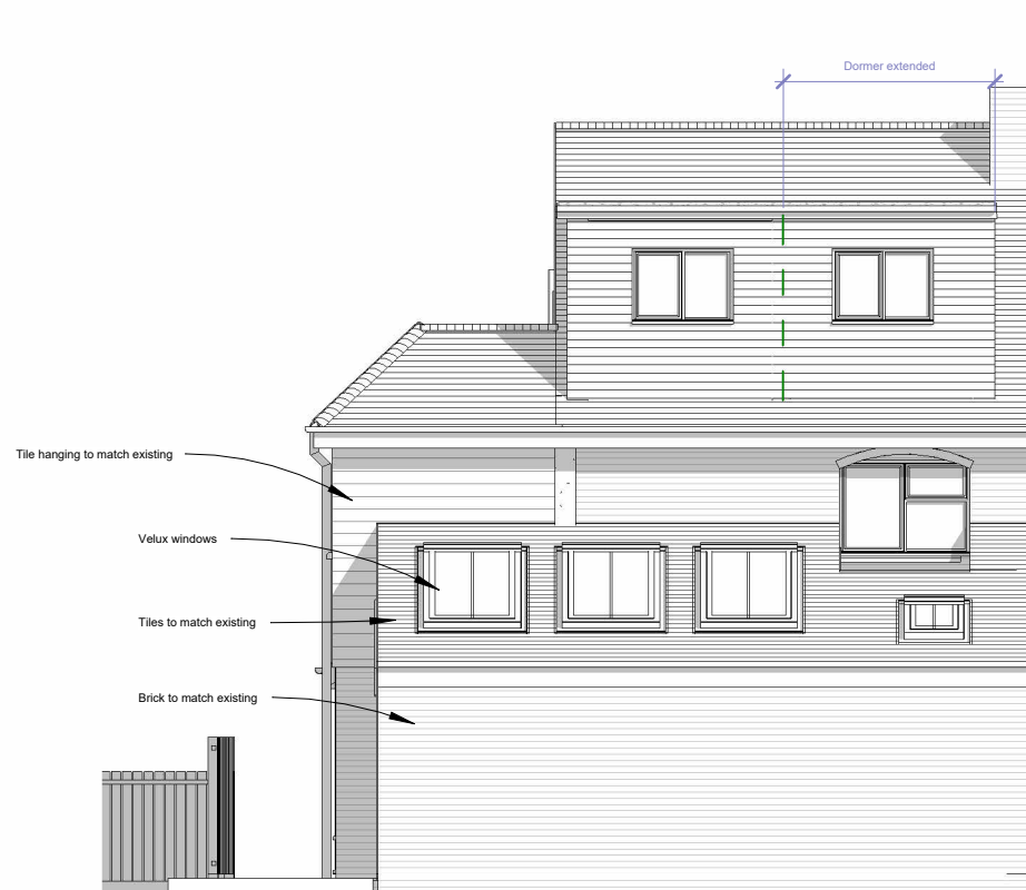
4 Proposed West Elevation 1 : 100
