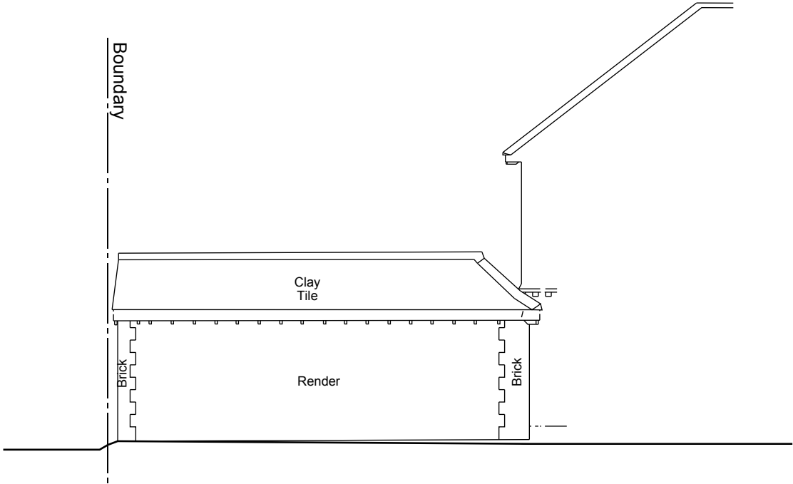
North Elevation
