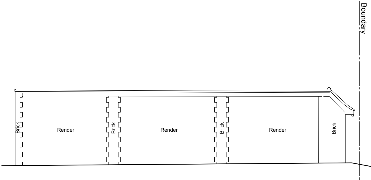
East Elevation
