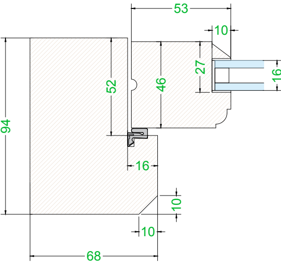
Frame Jambs & Casement Stiles Section Details Scale: 1:2 @ A3
