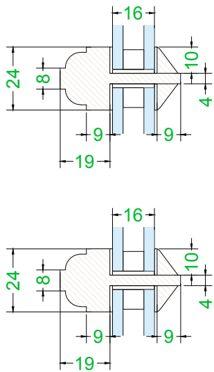
Frame Cill & Casement Bottom Rail Section Details Scale: 1:2 @ A3
