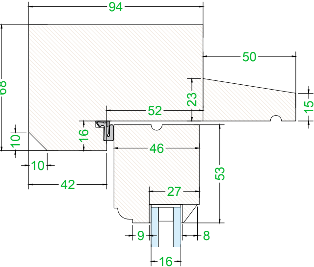
Glazing Bar Section Details Scale: 1:2 @ A3
