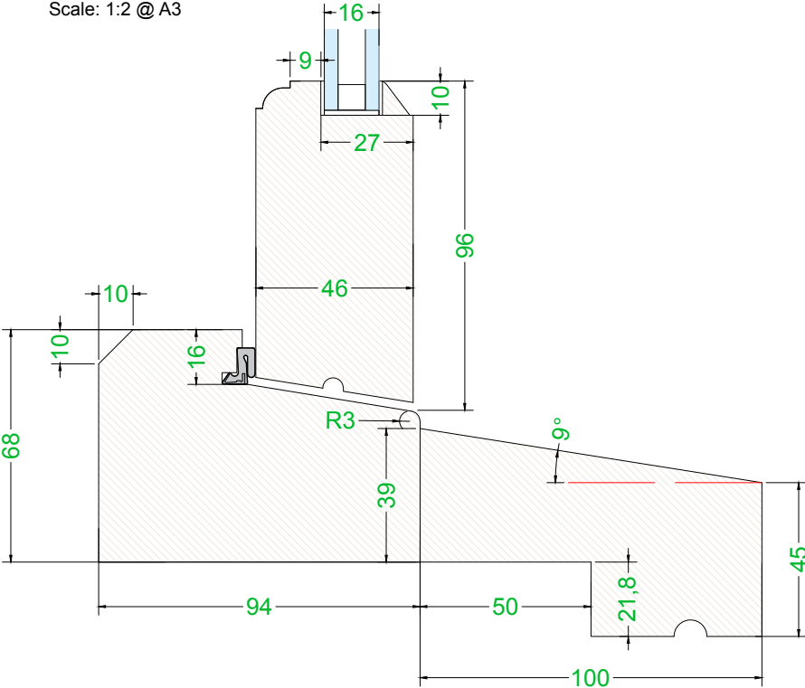
Frame Cill & Casement Bottom Rail Section Details Scale: 1:2 @ A3
