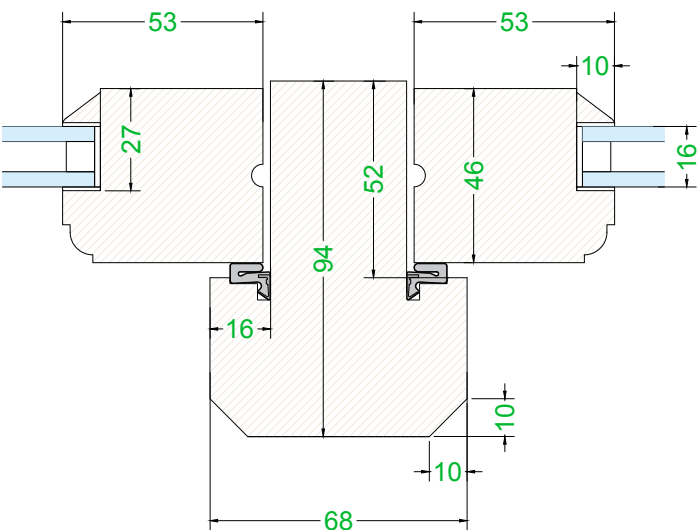
Frame Mullion & Casement Stiles Section Details Scale: 1:2 @ A3
