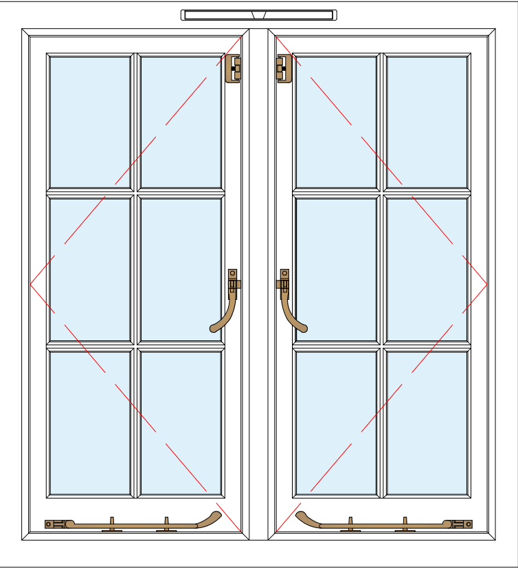
Double Casement Window As Viewed Internally Scale: 1:10 @ A3
