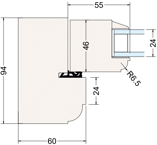
Frame Head / Jamb & Casement Stile Section Detail Scale: 1:2 @ A3
