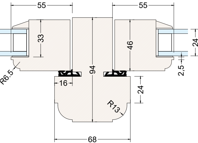
Frame Mullion & Casement Stiles Section Detail Scale: 1:2 @ A3
