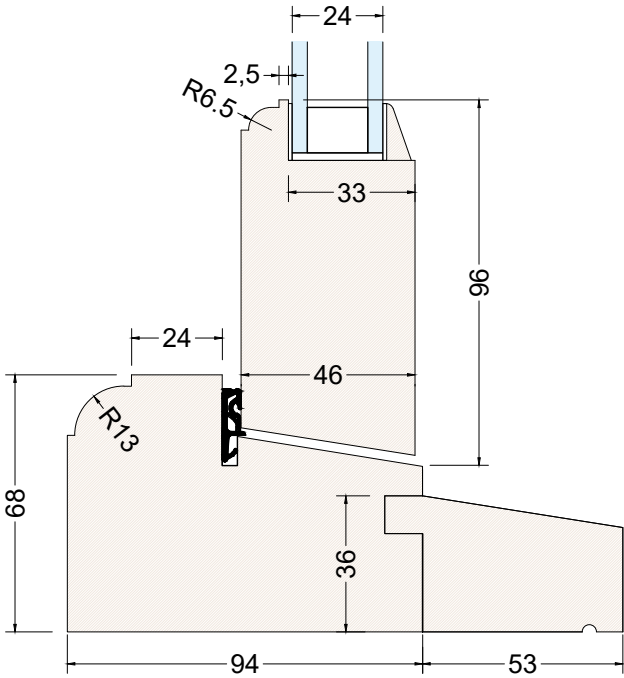
Frame Sill, Add On Sill & Casement Bottom Rail Section Detail Scale: 1:2 @ A3
