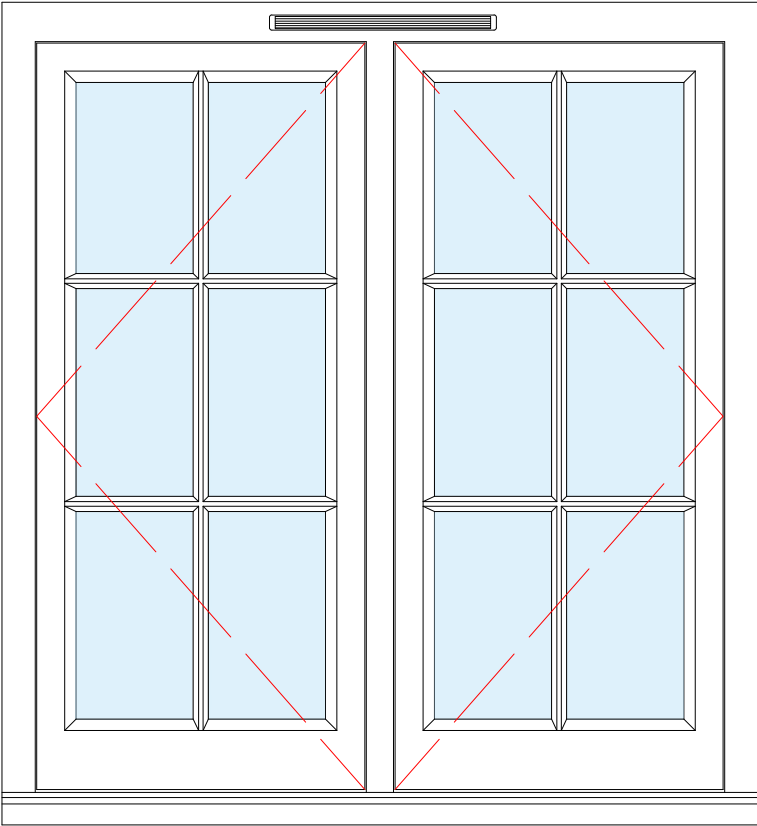
Double Casement Window As Viewed Externally Scale: 1:10 @ A3
