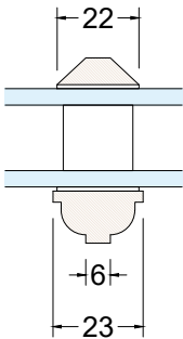
Glazing Bar Section Detail Scale: 1:2 @ A3
