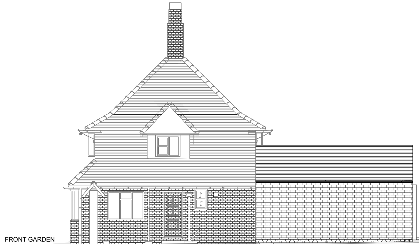
Part Side Elevation
