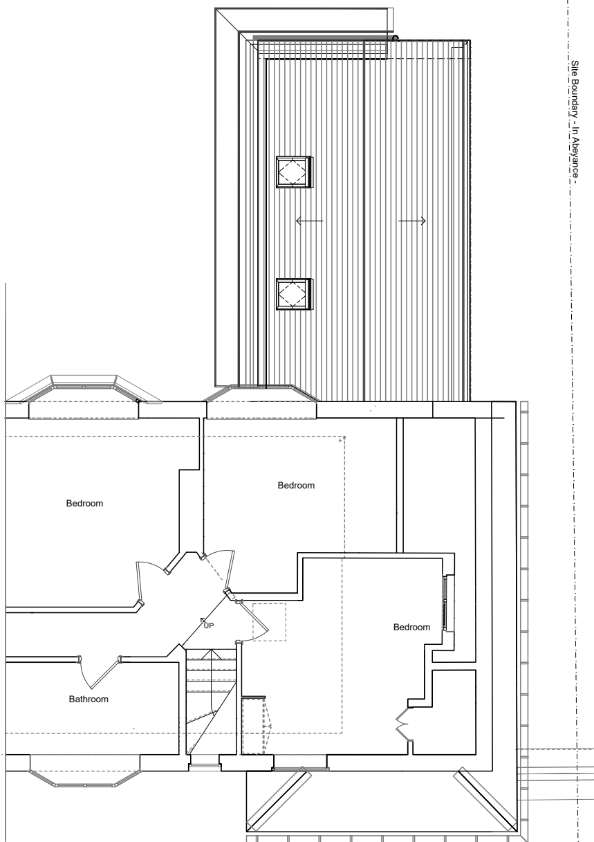
Part First Floor
