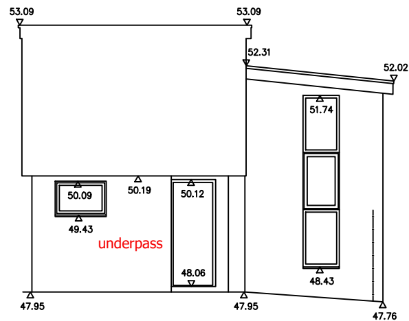
9.Existing South East Elevation (Studio GF underpass)
