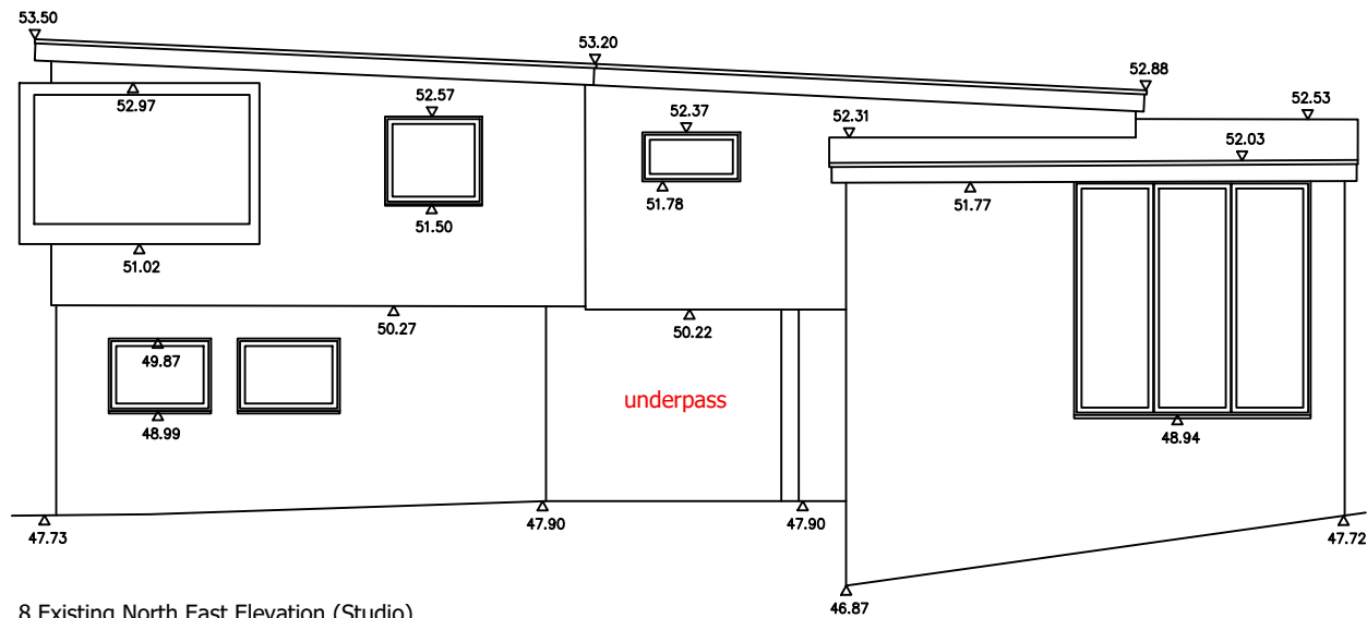
8.Existing North East Elevation (Studio)
