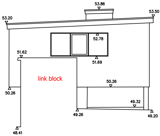
5.Existing South West Elevation (Studio)
