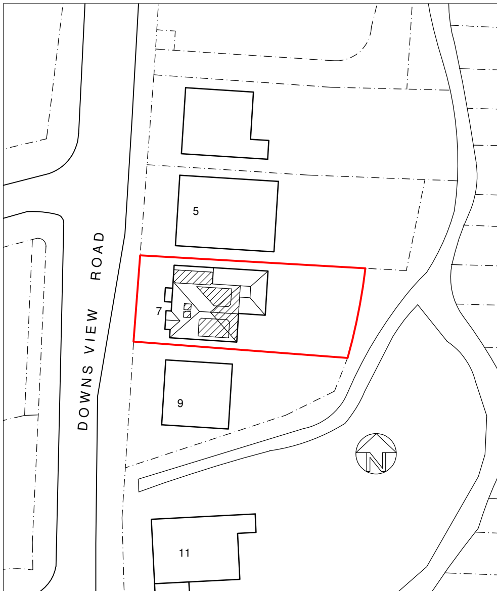
Block Plan 1:500
