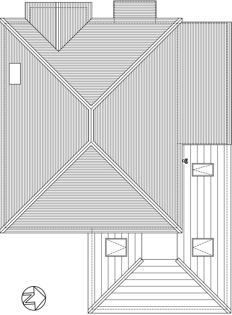
ROOF PLAN
