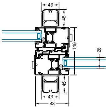
Standard Mullion with Internal and External Reinforcement
