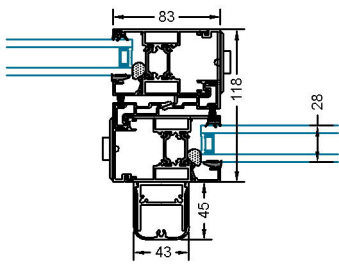
Standard Mullion with Internal Reinforcement
