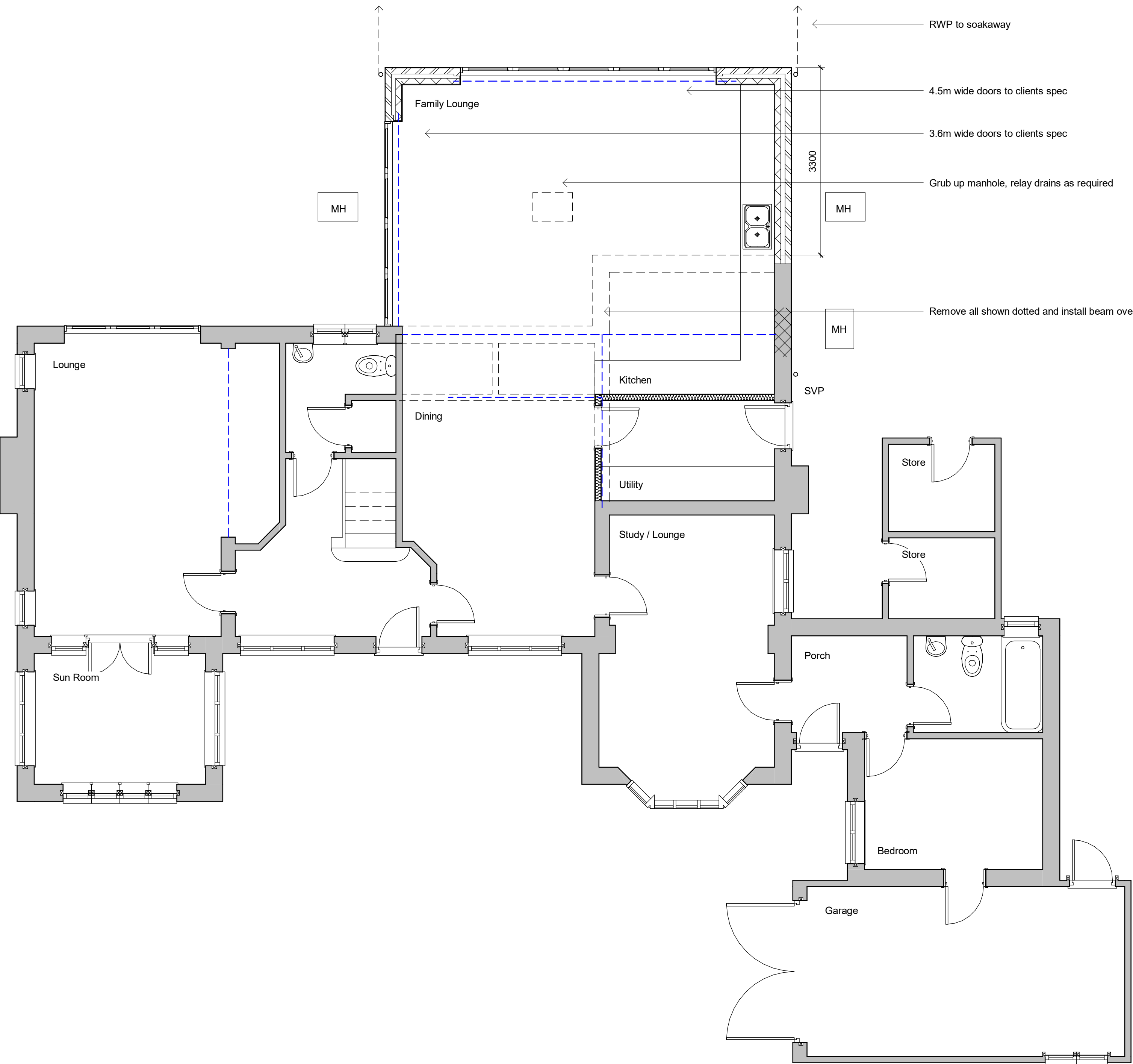
Ground Floor - Proposed - 1:50
