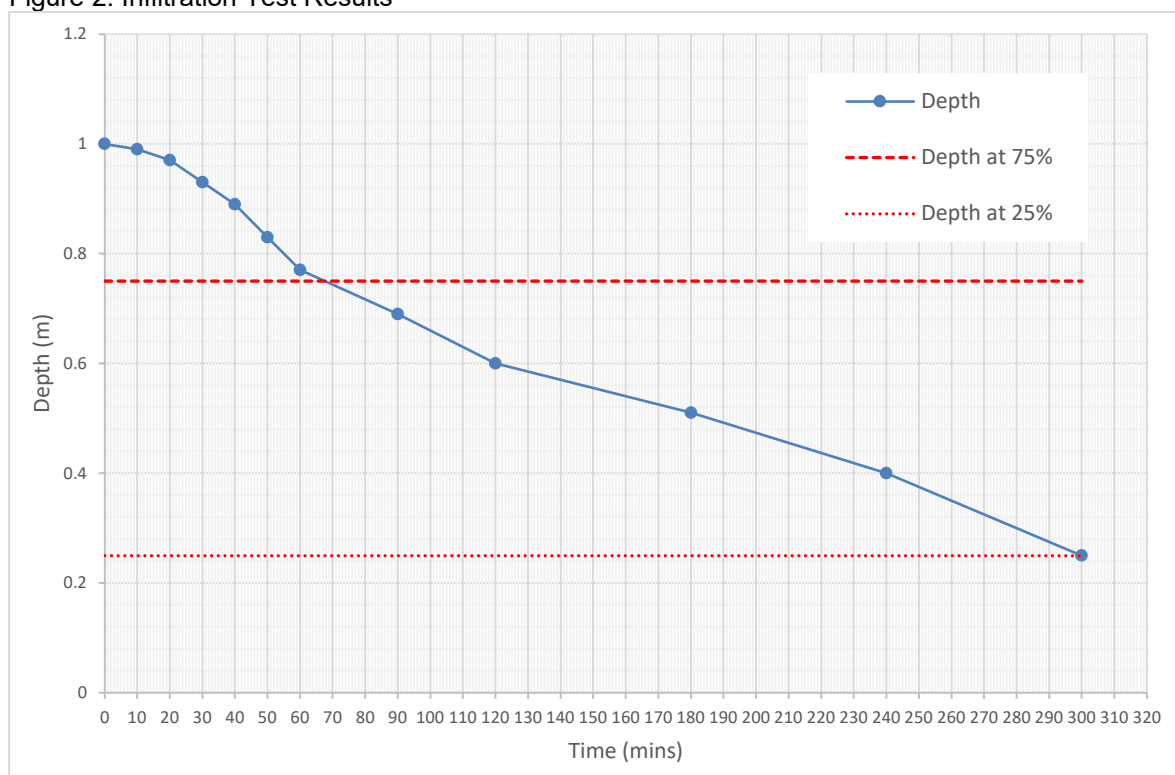
Figure 2: Infiltration Test Results
