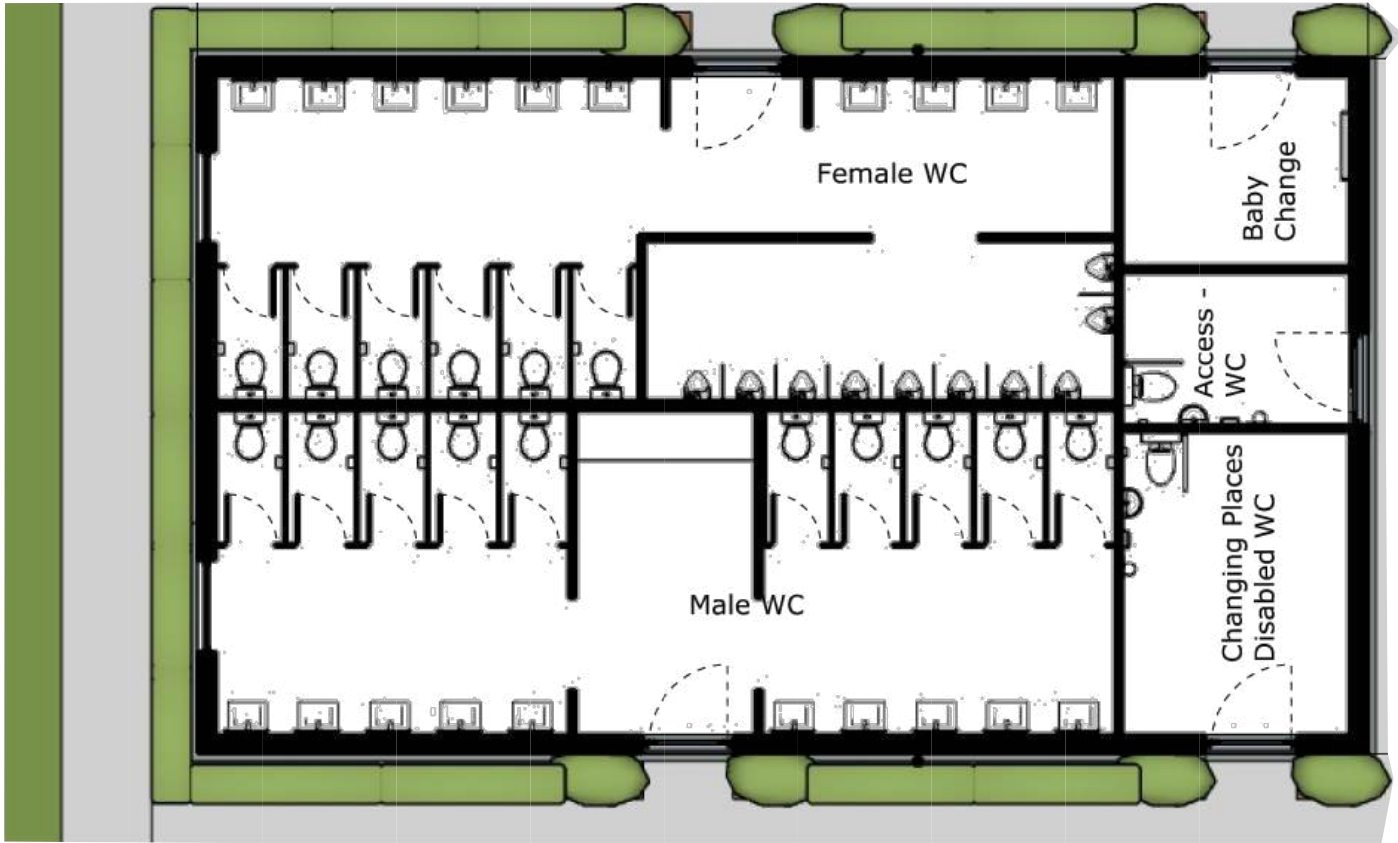
Proposed Plan 1:100
