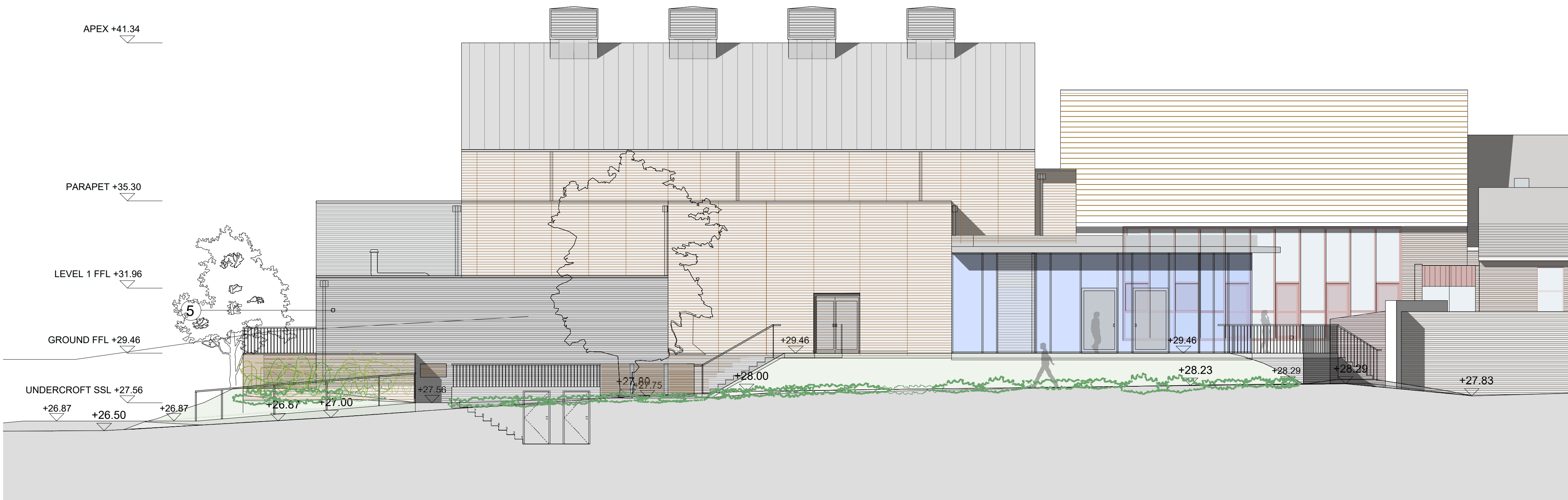
SOUTHERN ELEVATION
