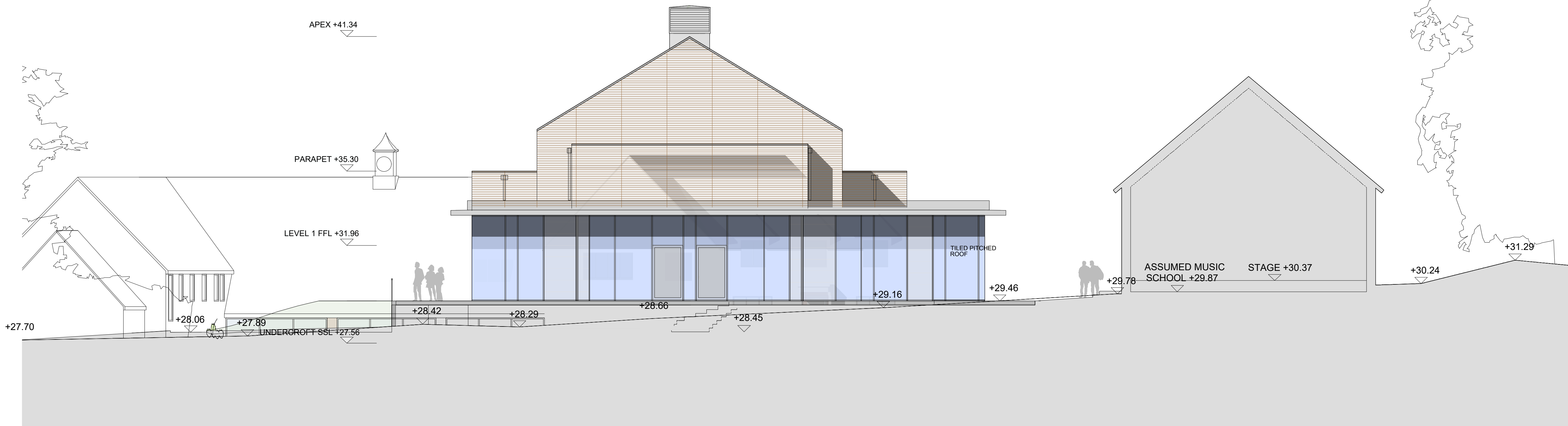
EASTERN ELEVATION
