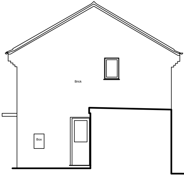
4 - North-West Elevation
