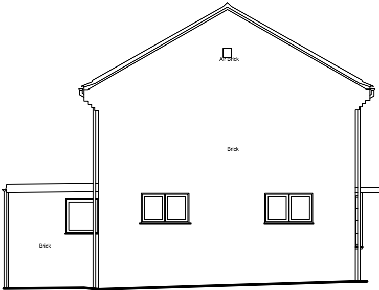
2 - South-East Elevation
