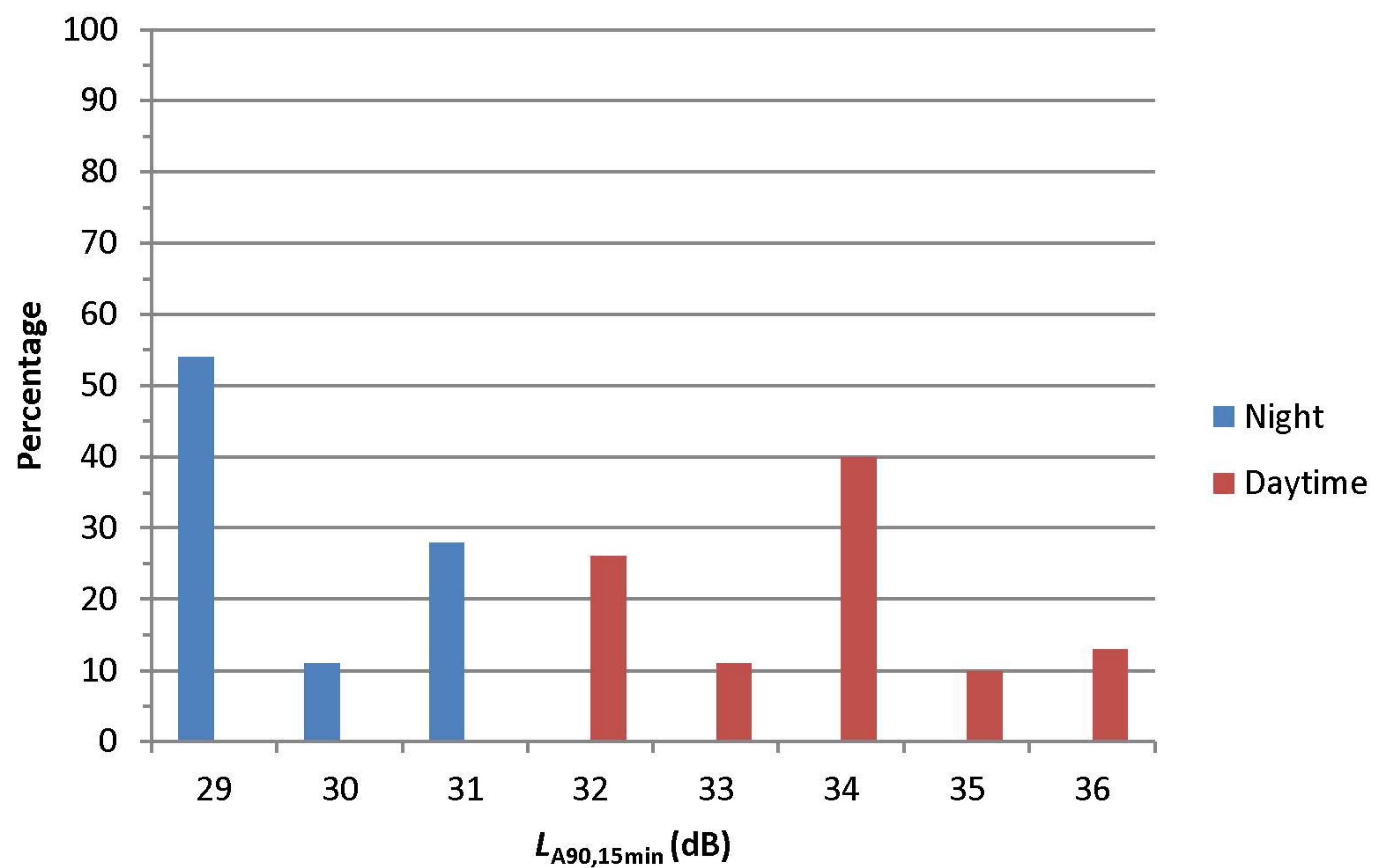
Figure 7.2 Histogram of background sound levels ( L_{A90,15min} )
