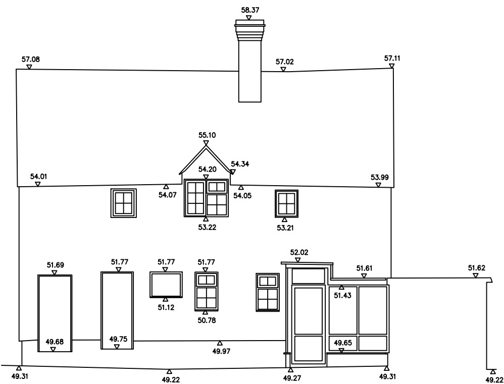
4.Existing North East Elevation (Main House)
