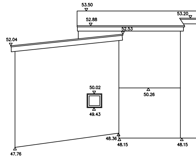
7.Existing North West Elevation (Studio)
