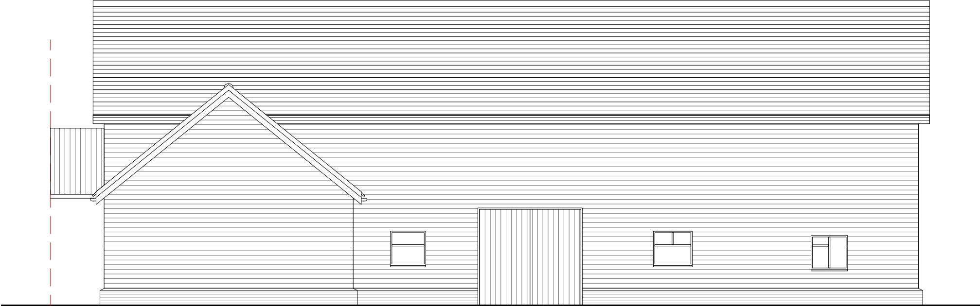
South West Elevation - Existing Scale 1:100
