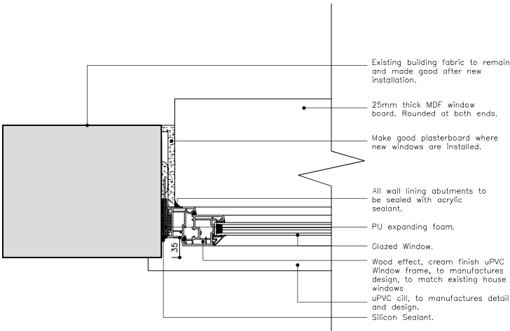
WINDOW JAMB DETAIL REPLACEMENT WINDOWS
