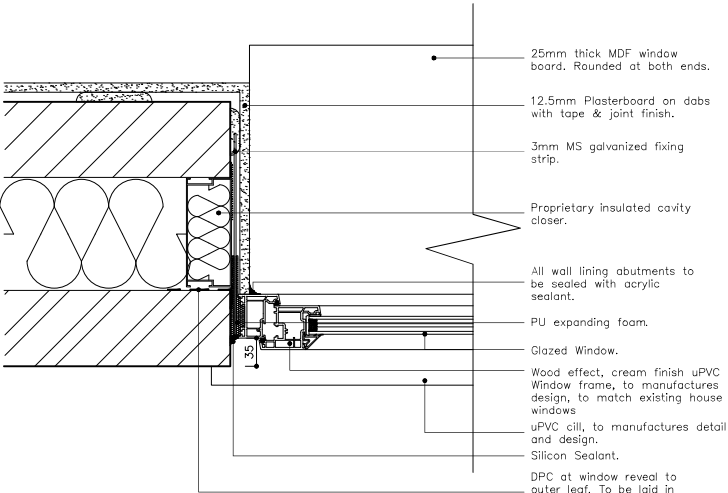
WINDOW JAMB DETAIL NEW EXTENSION
