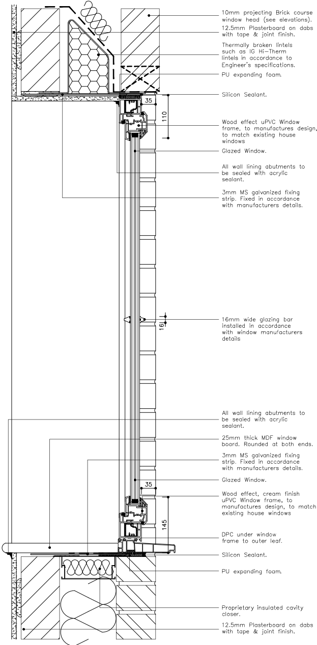
WINDOW SECTION HEAD & CILL DETAIL
