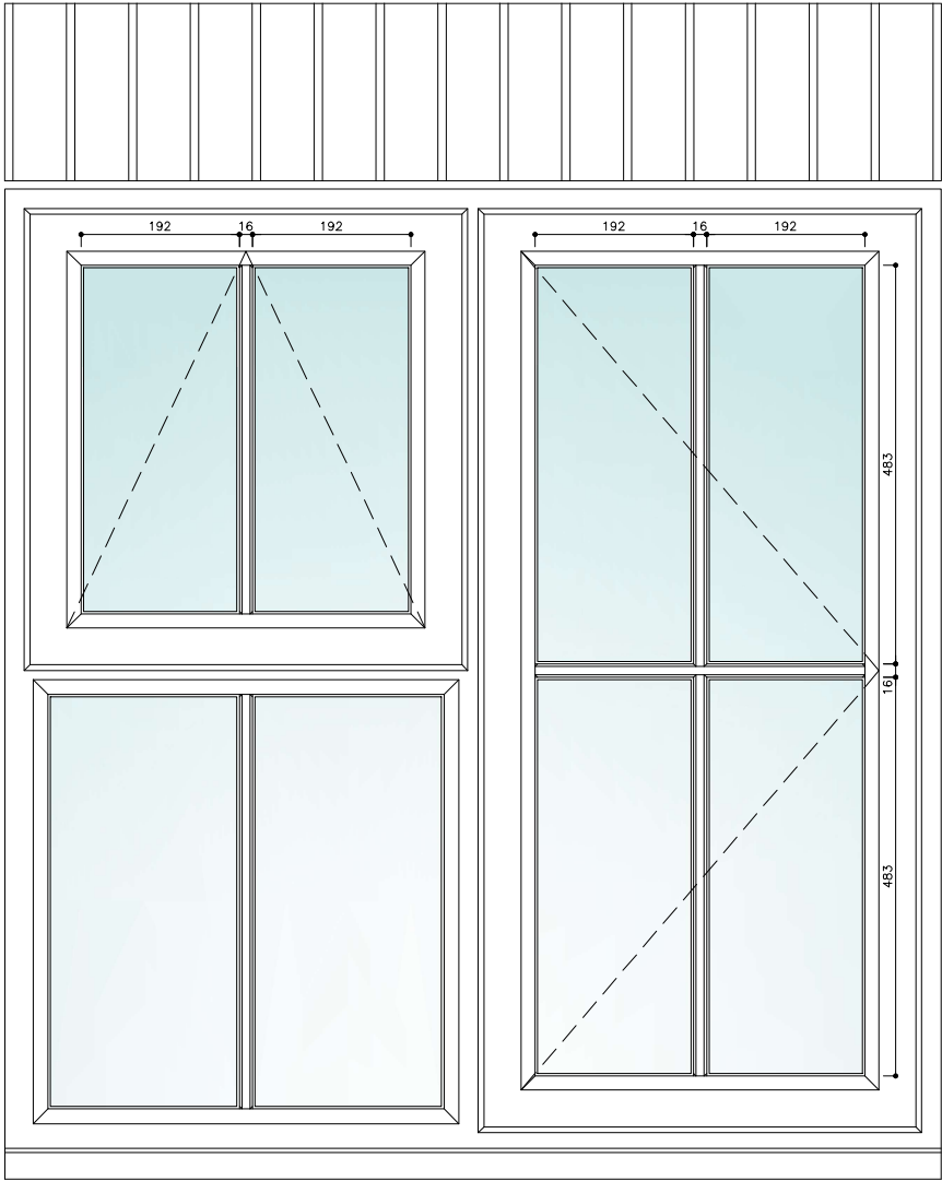
TYPICAL WINDOW ELEVATION
