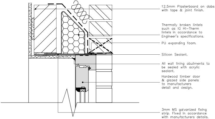
DOOR SECTION HEAD DETAIL
