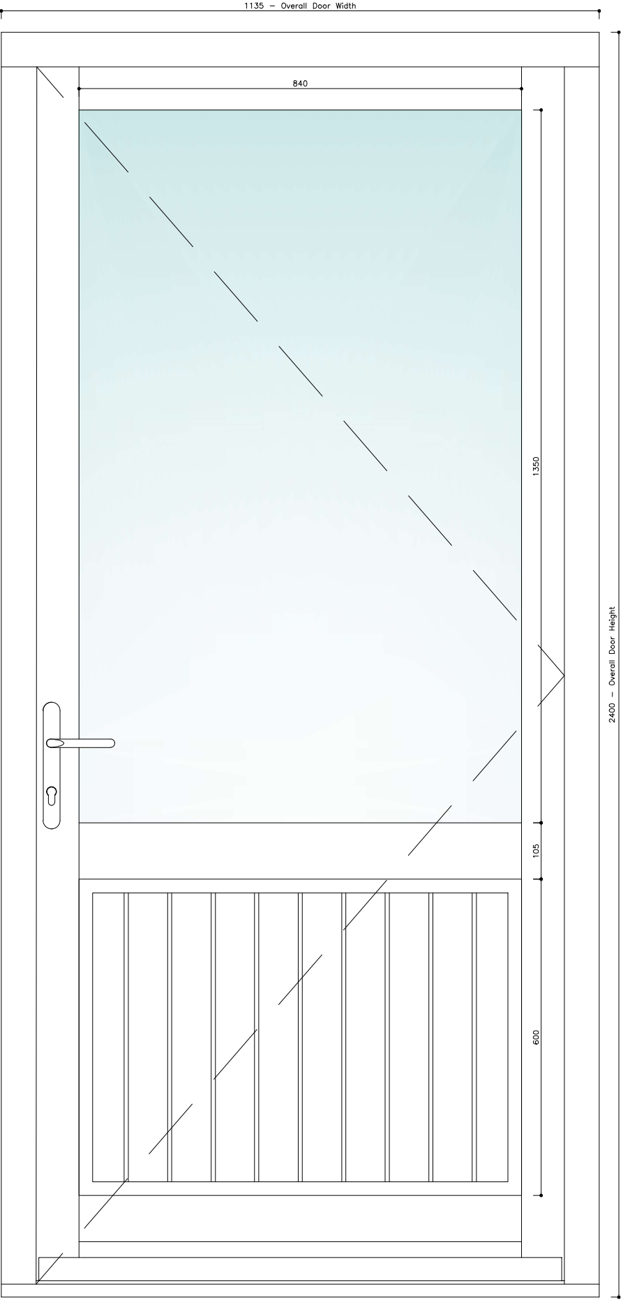
TYPICAL TIMBER DOOR ELEVATION
